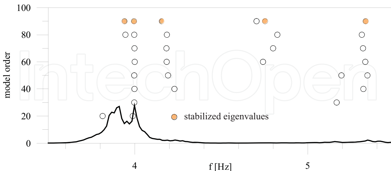
Fig. 10. Eigenvalue stabilization diagram for the Vallone Scarpa bridge.
