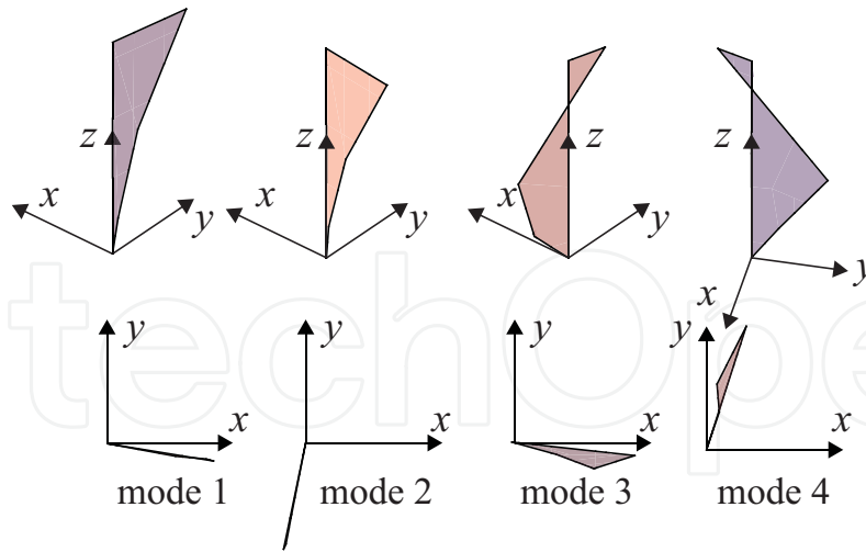
Fig. 5. Experimental mode shapes.
