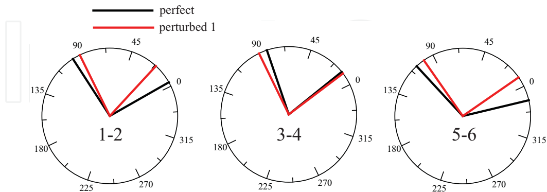
Fig. 6. Top view of the experimental mode shapes of a clamped pipe.
