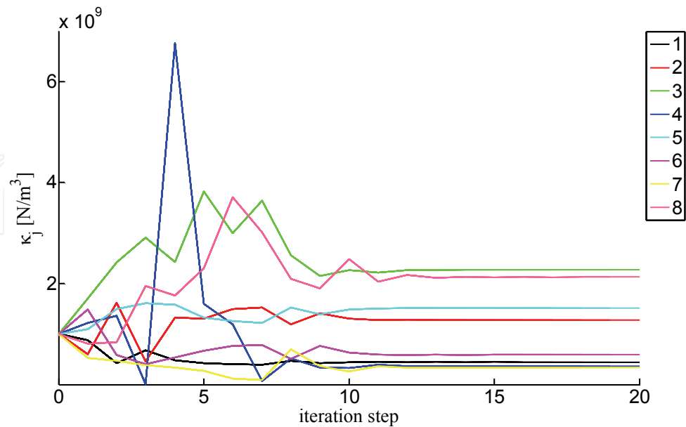
Fig. 18. Evolution of stiffness parameters \kappa_j ( j=1, \dots, 8 in the legend) during iterations by adopting the proposed updating procedure. Example with 4 measurement response dofs and with 10% noise.
