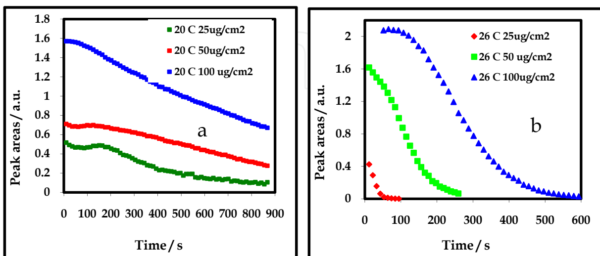
Fig. 21. Plots of peak areas versus time (second) for 25, 50 and 100 \mu\text{g}/\text{cm}^2 at a: 20 °C; b: 26 °C
