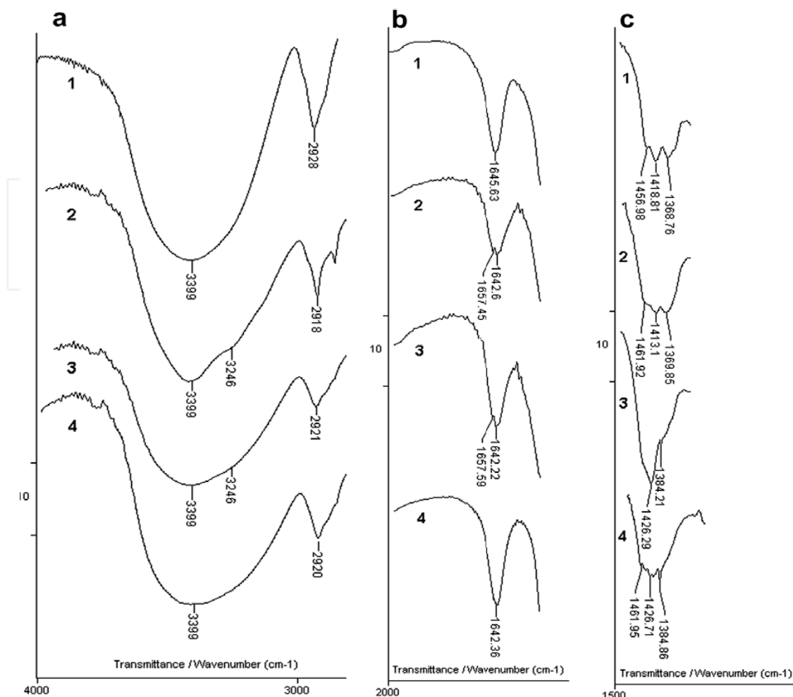
Fig. 4. Stretching (a), bending in plane (b) and bending in plane OH plane (c) region from LNT-FTIR spectra of RLMP (1) and synthesized Cu(II)-RLMP complexes at boiling point and pH 8.0 (2), 10.0 (3), 12.0 (4)
