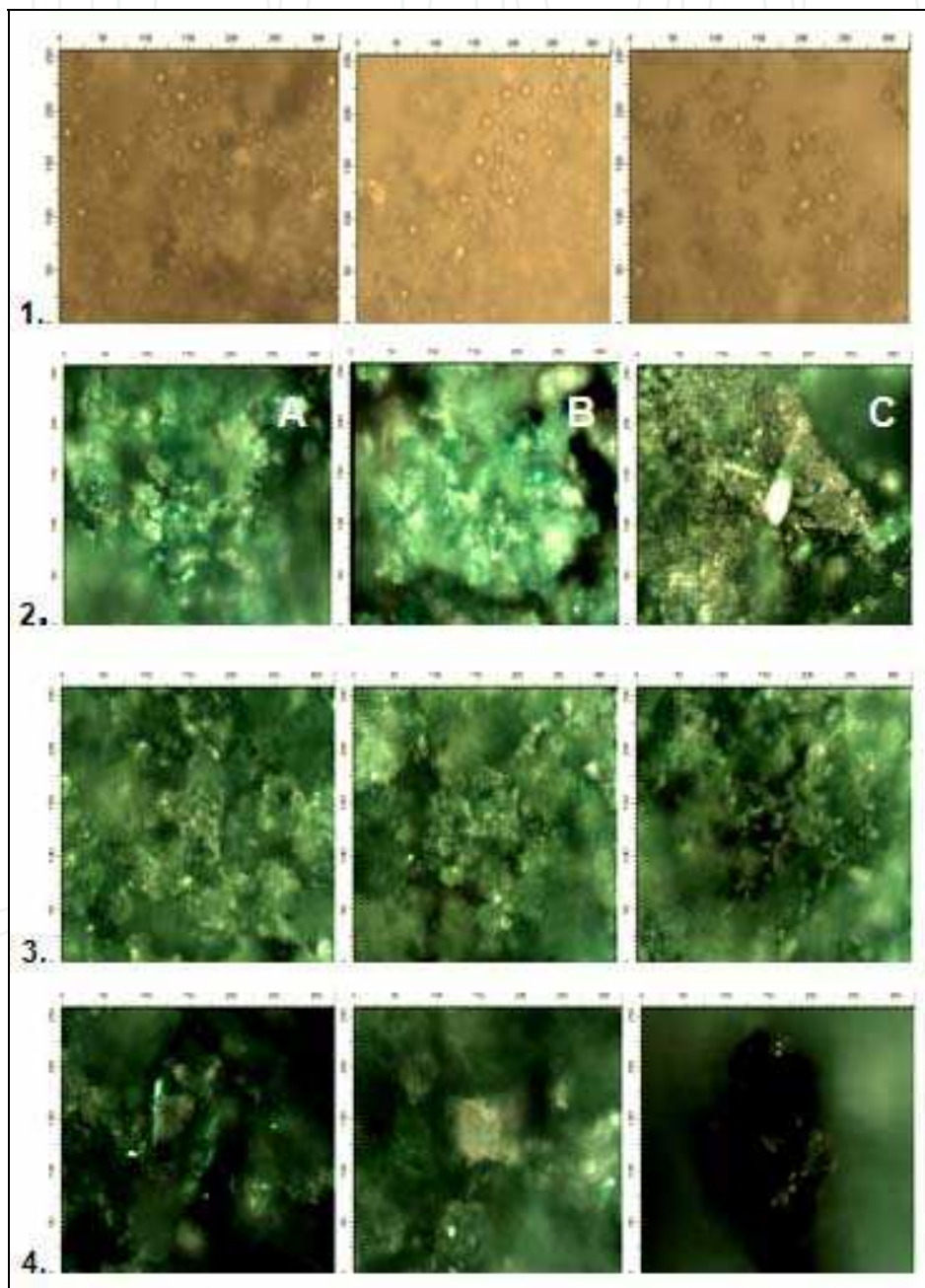
Fig. 14. FTIR microscopy images ( 250\ \mu\text{m} \times 300\ \mu\text{m} ) of RLMD, M_w = 5.000\ \text{g mol}^{-1} (1) and Cu(II) complexes with RLMD synthesized at boiling point and pH 7-8 (2), 8-10 (3) and 10-12 (4)
