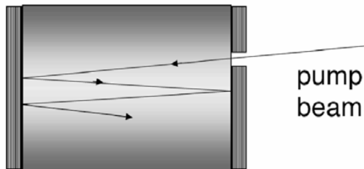
Fig. 2.3. Mirrored sample multiple-pass scheme (figure from ref. [4])
