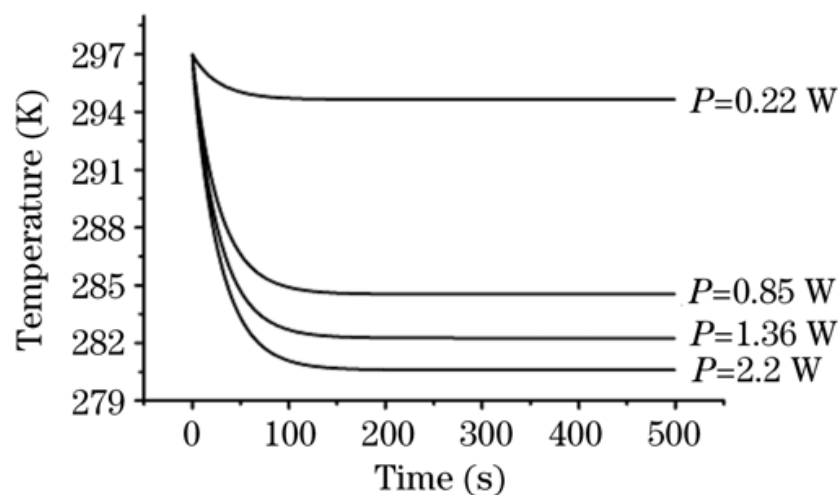
Fig. 3.3. Temperature drop with different pump laser power (Figure from ref. [16])
