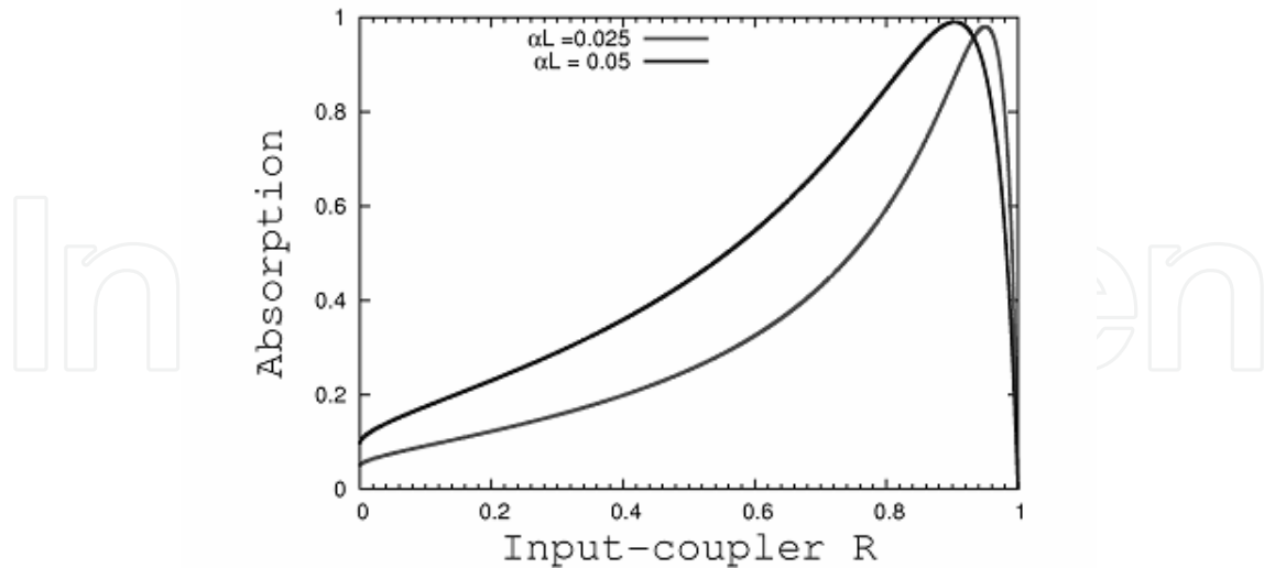
Fig. 4.4. The relationship between the cavity-enhanced absorption and the input-coupler reflectivity for two different values of \alpha l (Figure from ref. [13])
