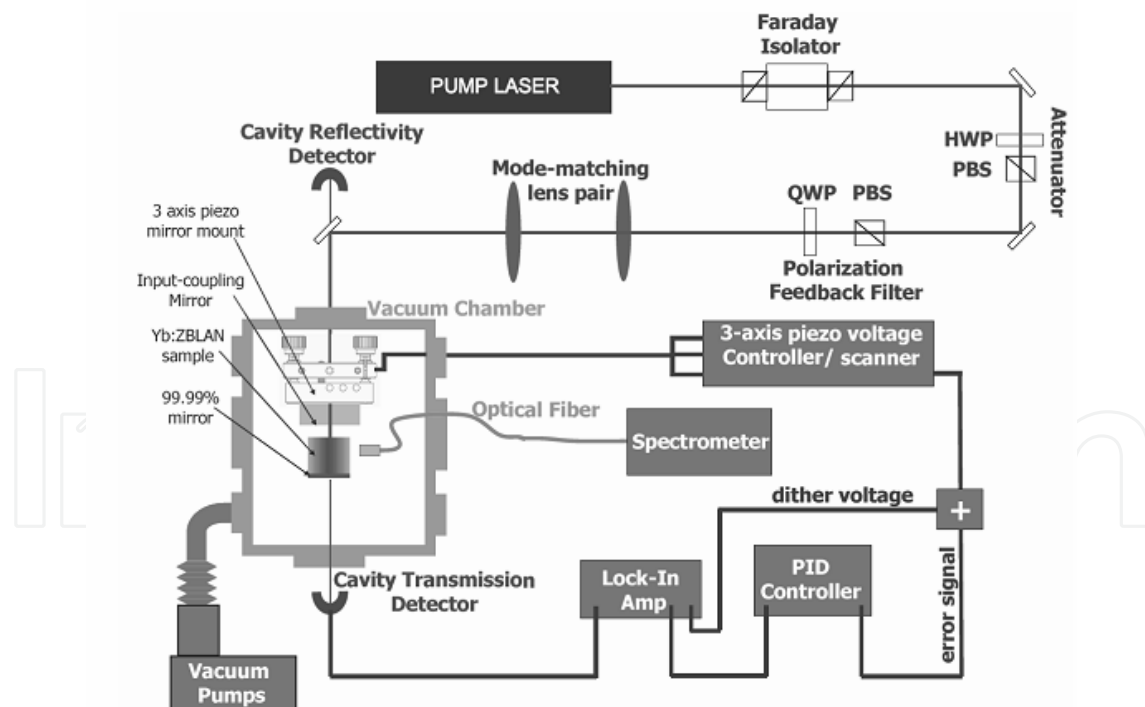
Fig. 4.7. Experimental setup of extra-cavity resonant enhancement scheme for laser cooling of solids. The thin lines are the optical beam path, and the thicker lines are electronic connections. (Figure from ref. [10])
