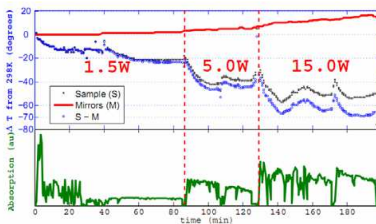
Fig. 4.9. The top graph shows the temperature dynamics \Delta T (offset to zero at 298K). The grey closed circles, the red solid line and the blue open circles represent the temperature change of the sample, cavity mirrors and the difference temperature of the chamber and sample, respectively. The bottom graph is the absorption on linear scale in arbitrary units. (Figure from ref. [17])
