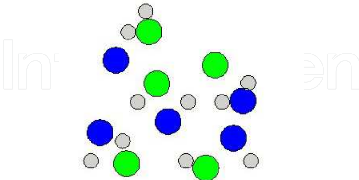
Fig. 21. Plane view of TlGaTe_2 and TlInTe_2 after (Matsumoto et al., 2008). The green, blue and gray balls represent Ga or In, Tl and Te atom respectively.
