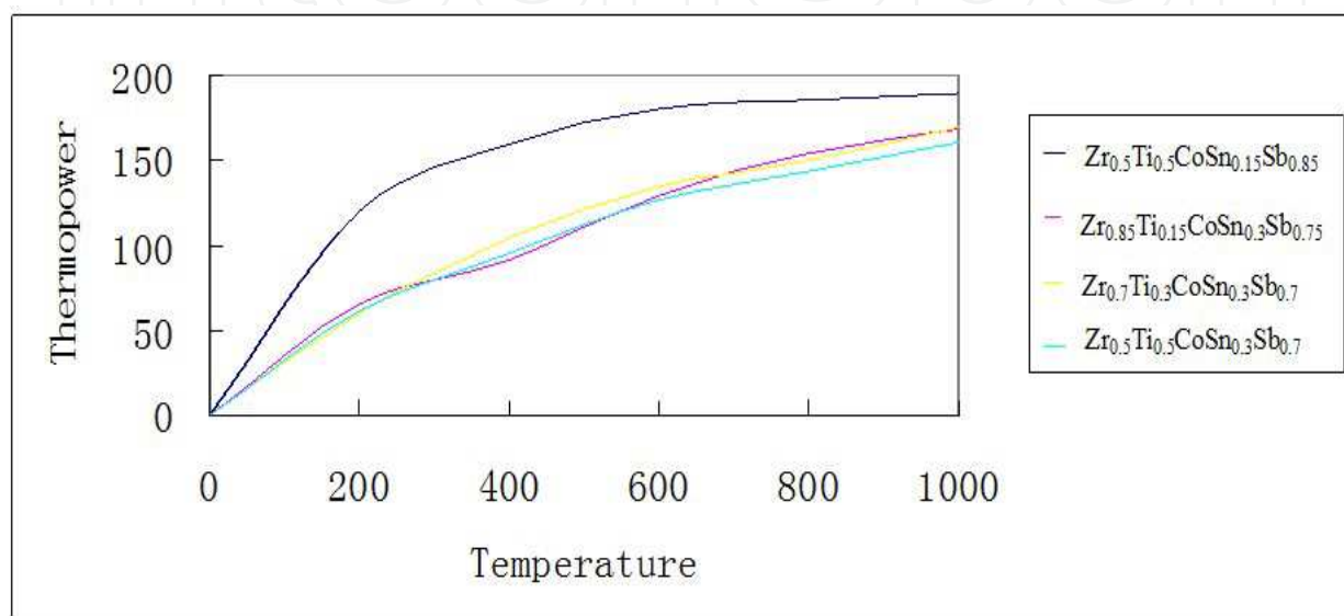
Fig. 27. Relations between thermopower ( \mu\text{V}/\text{K} ) and temperature (K) for Ti content varied \text{Zr}_{1-x}\text{Ti}_x\text{CoSn}_{0.3}\text{Sb}_{0.7} series and Sn content reduced \text{Zr}_{0.5}\text{Ti}_{0.5}\text{CoSn}_{0.15}\text{Sb}_{0.85} alloy. Data source from (Ponnambalam et al., 2008)
