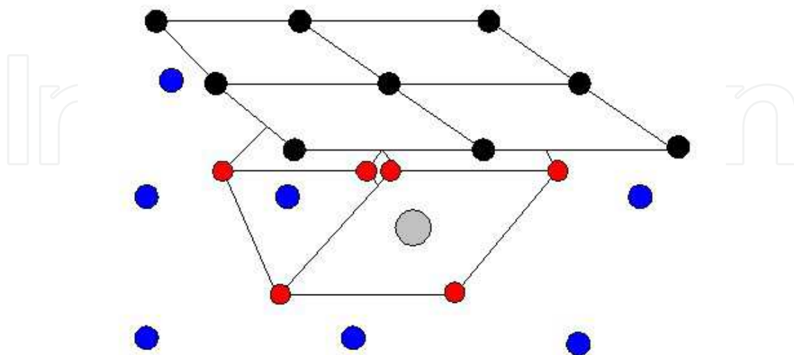
Fig. 8. \text{YbZn}_{2-x}\text{Mn}_x\text{Sb}_2 structure view after (Yu et al., 2008). Black spheres denote Yb atoms, red spheres denote Sb atoms, blue spheres denote Zn atoms and gray sphere denotes Mn atom.
