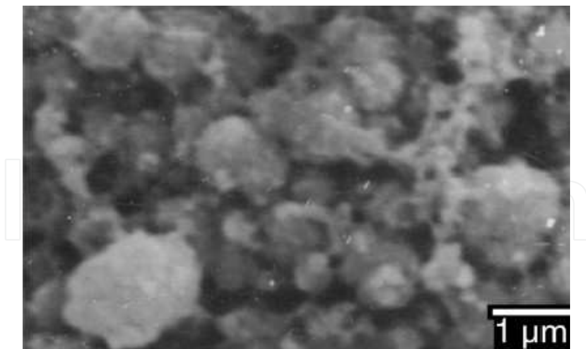
Fig. 29. SEM image of PANI/ Bi 2 Te 3 (10000 magnification). Reproduced from (Chatterjee et al., 2009)
