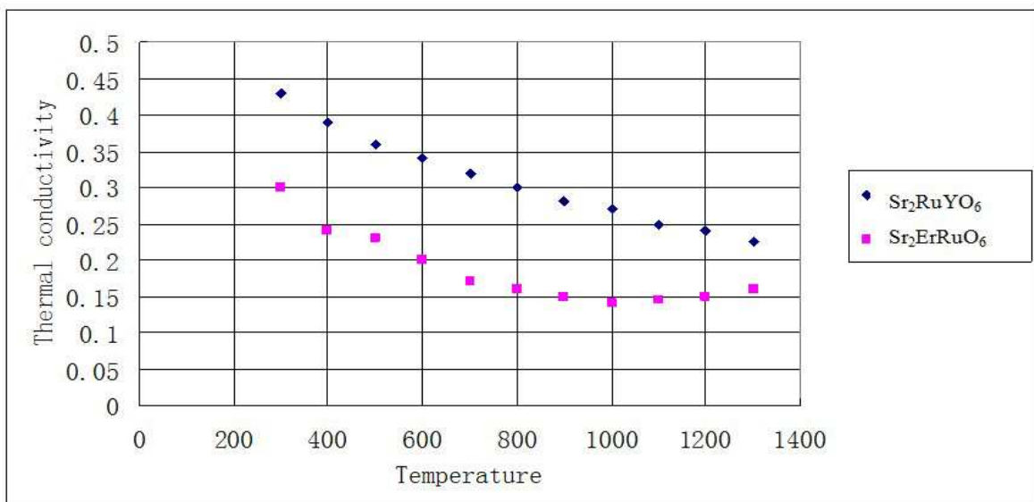
Fig. 26. The relations between temperature (K) and total thermal conductivity ( \text{W}\cdot\text{K}^{-1}\cdot\text{m}^{-1} ) for \text{Sr}_2\text{RuYO}_6 & \text{Sr}_2\text{ErRuO}_6 . Data source from (Aguirre et al., 2005).
