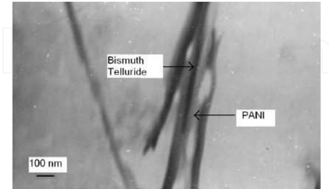
Fig. 28. TEM images of PANI/Bi 2 Te 3 composite. Reproduced from (Chatterjee et al., 2009)
