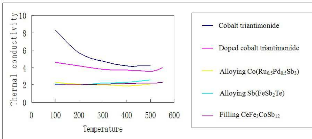
Fig. 14. Reduced thermal conductivity ( \text{W K}^{-1} \text{m}^{-1} ) with different doping and filling materials at different temperatures ( ^{\circ}\text{C} ). Data source from (Snyder & Toberer, 2008).
