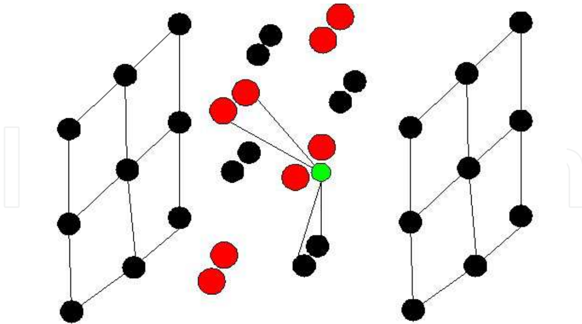
Fig. 20. Crystal structure of Ce_{1-x}Cu_xSe_2 after (Rhyee et al., 2010). Black spheres denote Se atoms, red spheres denote Ce atoms and green sphere denotes Cu atom.
