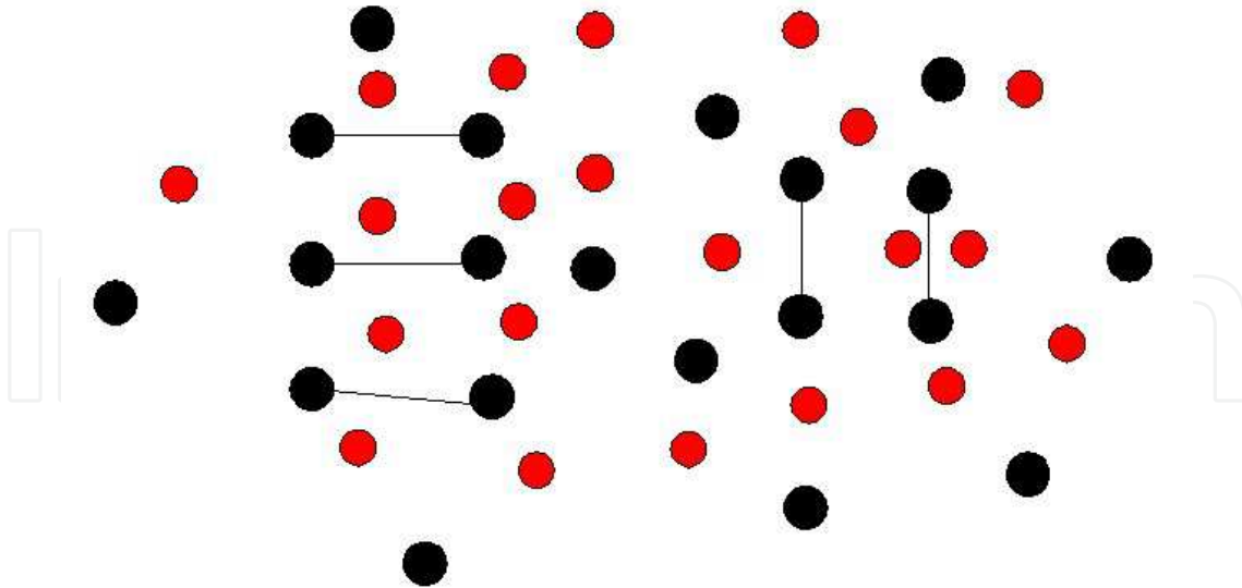
Fig. 11. Layered view of three distinct types of Sb atoms in X_{11}Sb_{10} structure after (Kauzlarich et al., 2007). X is denoted by red sphere and Sb is denoted by black sphere.
