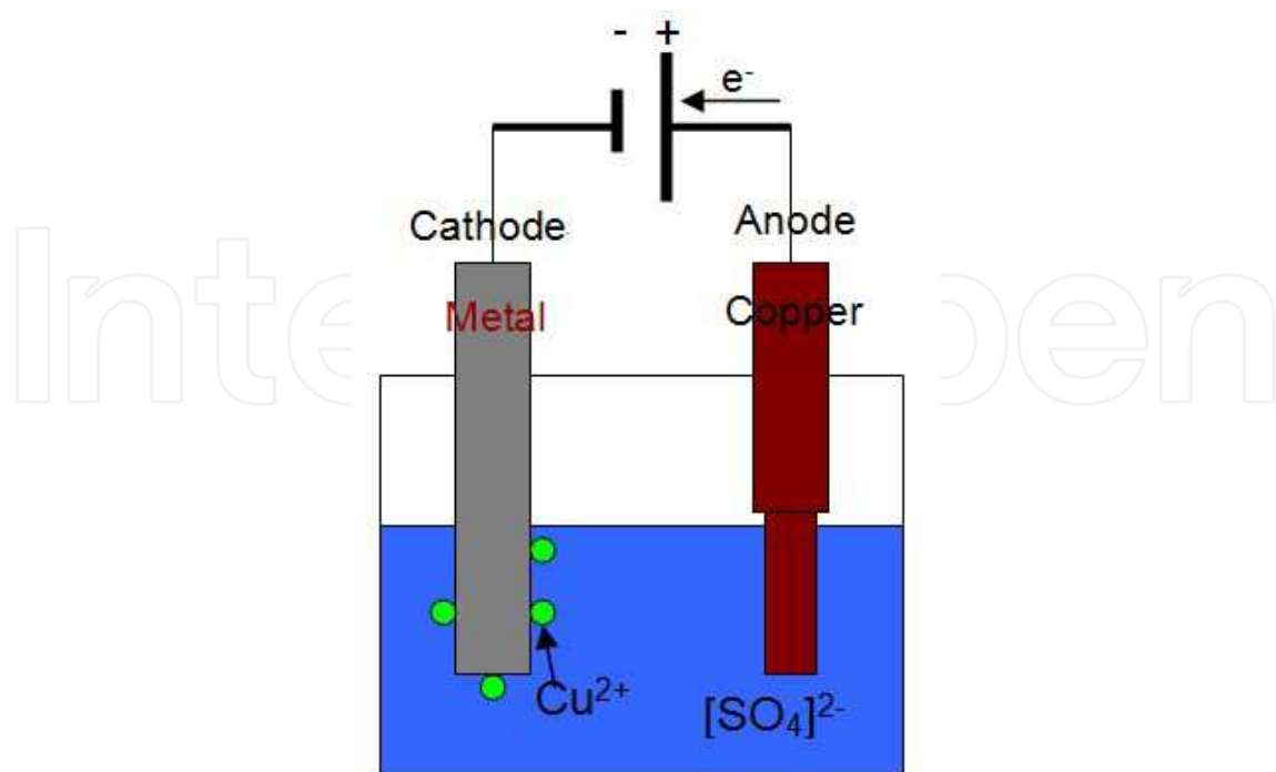
Fig. 3. Electroplating of a metal with copper in a copper sulfate bath.
