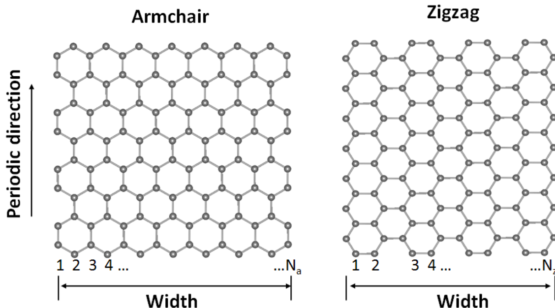
Fig. 1. Structure of armchair and zigzag nanoribbons
