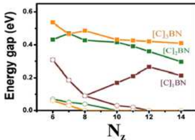
Fig. 16. The spin-resolved band gaps of hybrid BCN nanoribbons (Kan et al, 2008b).
