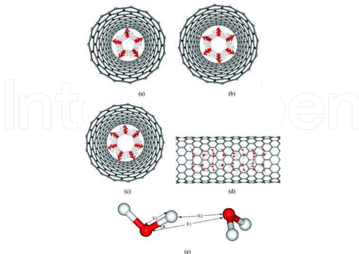
Fig. 6. Optimized (a) pentagonal, (b) hexagonal, and (c) heptagonal INT confined in zigzag ( l,0 ) SW-CNT, l = 15, 16, and 17, respectively, and (d) side view of hexagonal INT model; (e) structural parameters used for quantifying hydrogen bond as discussed in the text. Red, white, and gray spheres represent oxygen, hydrogen, and carbon atoms, respectively (Feng, Zhang et al. 2007).
