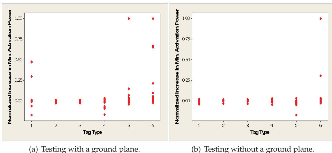
Fig. 2. The change in minimum activation power based on tag type. Two hundred sixteen tags were tested in the presence of a ground plane. One hundred sixty-two tags were tested without a ground plane. (©2007 IEEE (Bauer-Reich et al., 2007))
