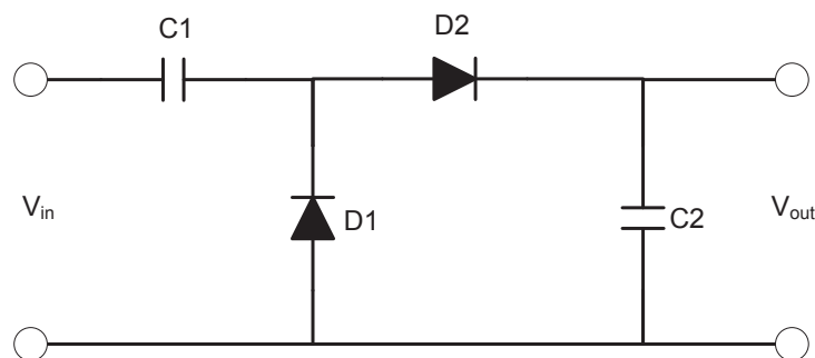
Fig. 1. Example Charge Pump
