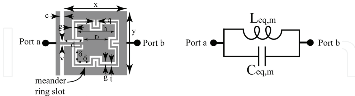
Fig. 7. (a) Layout of the MOCSRR particle (the gray area is the copper) and (b) the equivalent circuit of the MOCSRR particle.
