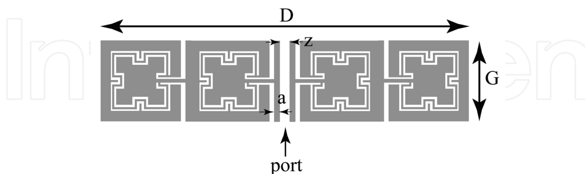
Fig. 9. Layout of the printed dipole using series connected MOCSRR particles (the gray area is the copper).
