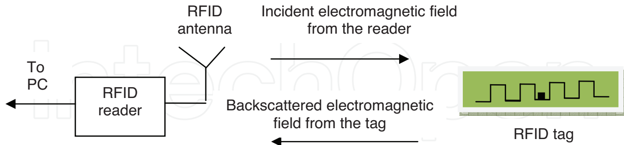
Fig. 1. Overview of a RFID system.
