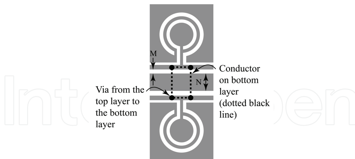
Fig. 5. CPW structure used to extract the equivalent circuit of the OCSRR particle (the gray area is the copper).
