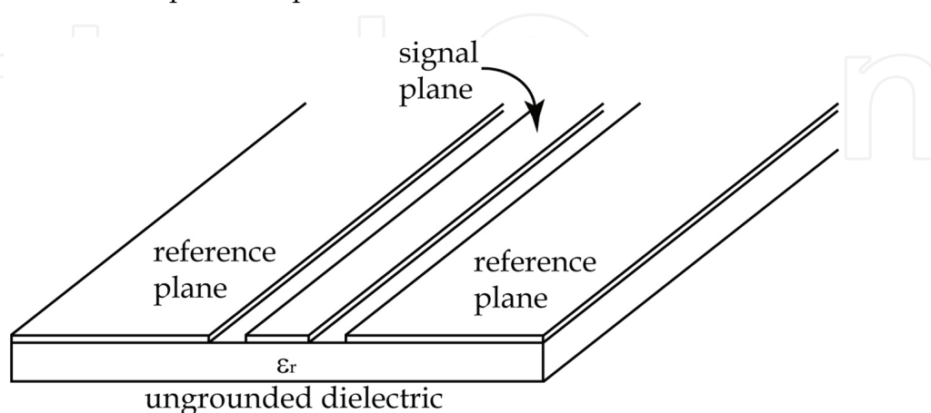
Fig. 2. A CPW transmission line on a dielectric substrate.
