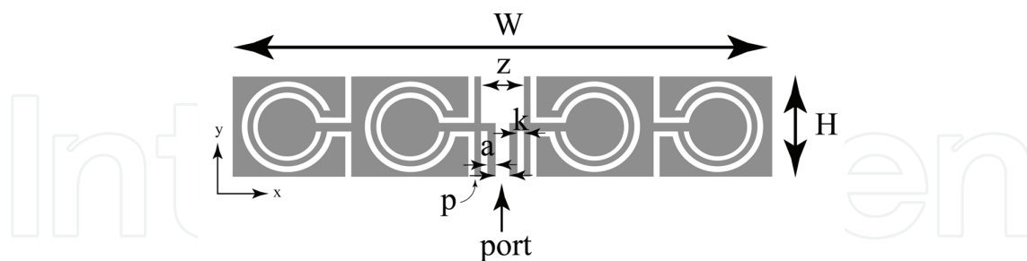
Fig. 6. Layout of the printed dipole using series connected OCSRR particles (the gray area is the copper).
