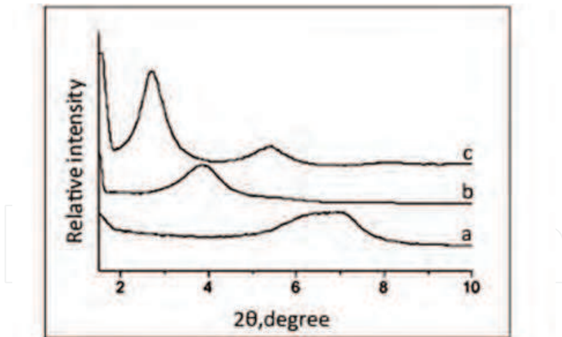
Fig. 4. XRD patterns of a) pristine sodium montmorillonite b) modified montmorillonite (OMT) c) ABS/OMT nanocomposite. ref:19
