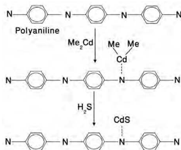
Fig. 1. Poly aniline/cadmium sulfide nanocomposite
