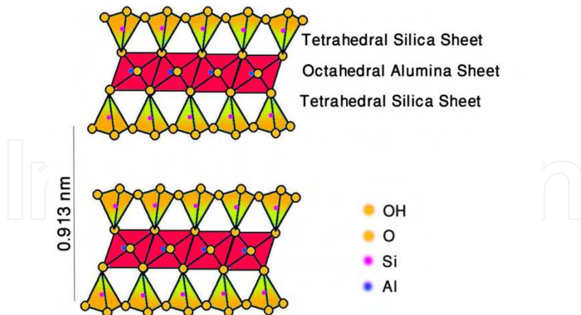
Fig. 10. Structure of pyrophyllite
