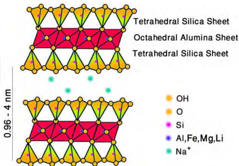
Fig. 11. Structure of sodium montmorillonite.
