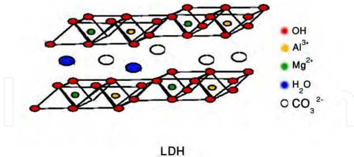
Fig. 14. Structure of layered double hydroxide
