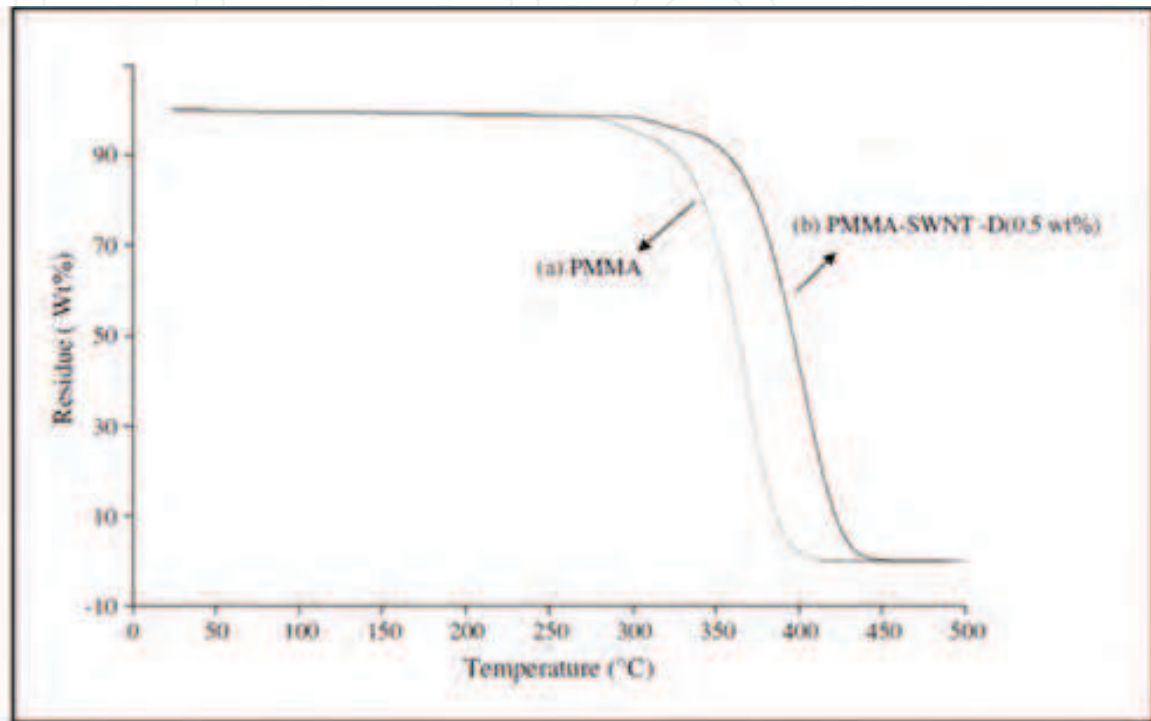
Fig. 15. TGA curves of a)PMMA b)PMMA/CNT nanocomposite ref:56
