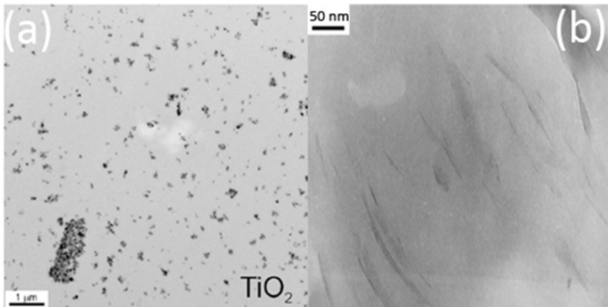
Fig. 5. TEM images of a) PMMA/TiO 2 nanocomposite b) ABS/OMMT nanocomposite ref:19,21
