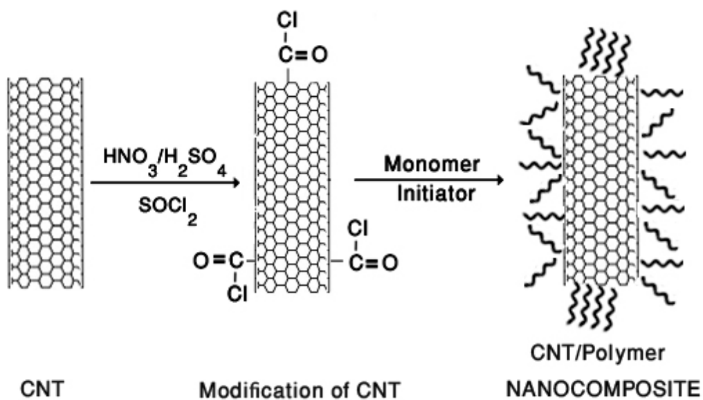
Fig. 16. Modification of carbon nanotube with organig agents
