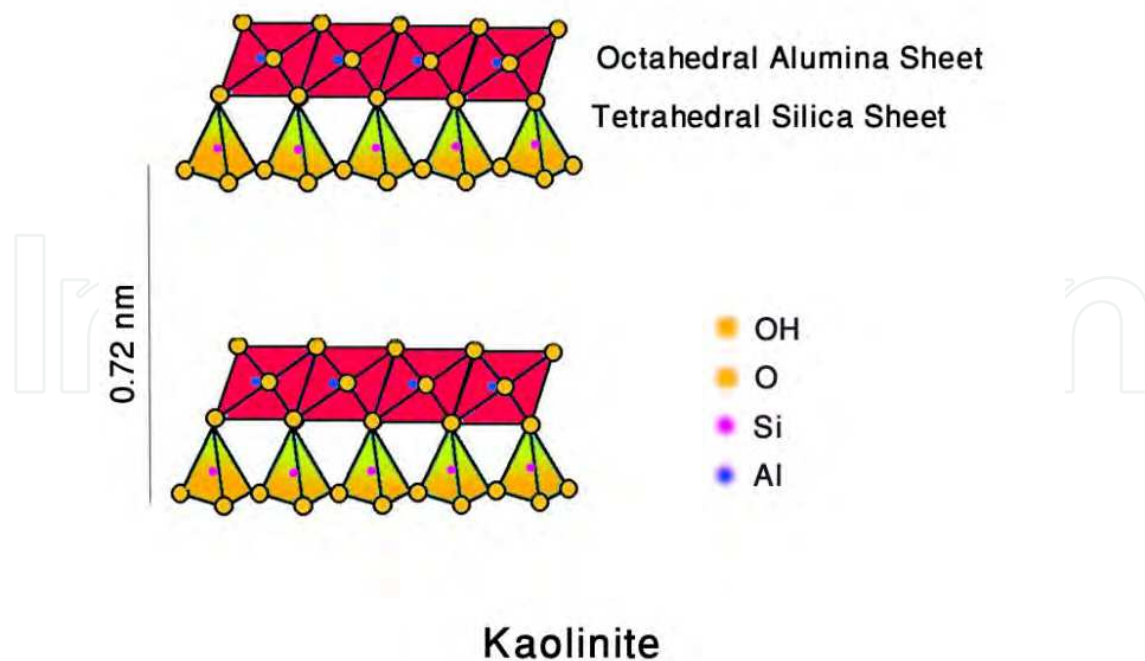
Fig. 9. Structure of kaolinite
