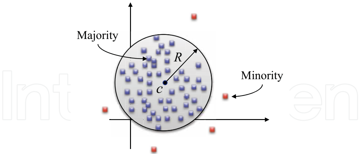
Fig. 6. The geometry of the sphere formulation of one-class SVM.
