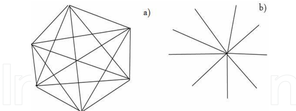
Fig. 4. The examples of networks with different node degree parameter values (a) Perfect graph of n nodes with avg. node degree n-1 . (b) Star graph of n+1 nodes with avg. node degree (2n)/(n+1)
