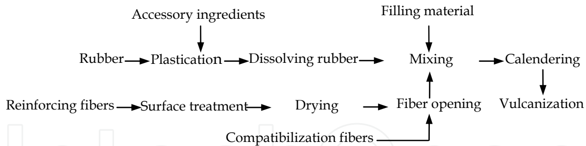
Fig. 3. A calender process of NASC
