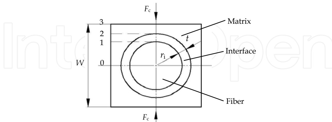
Fig. 16. A model of a compressive type single-fiber cell
