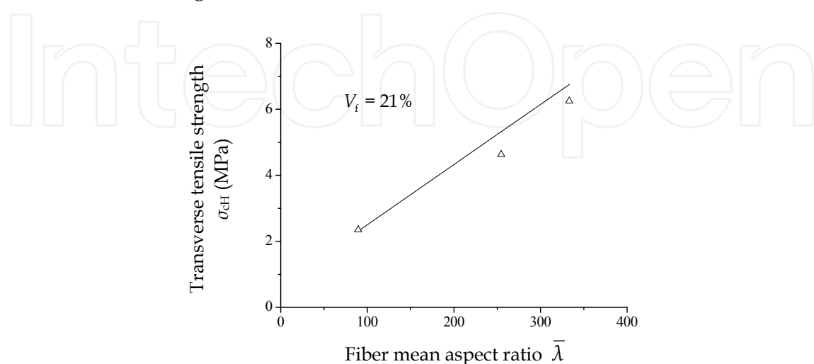
Fig. 20. Relationship between transverse tensile strength and fiber mean aspect ratio
