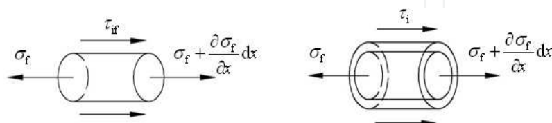
Fig. 13. Micromechanical stress transfer in NASC
