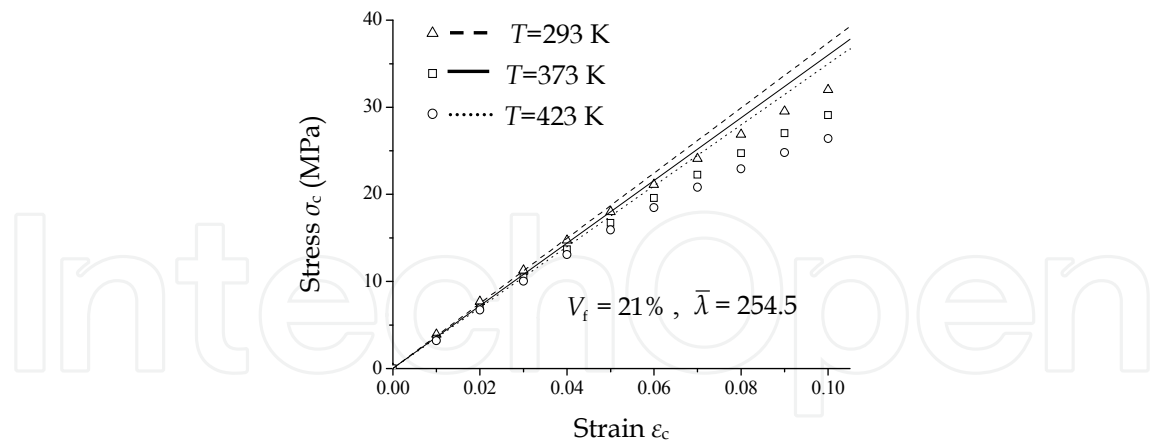
Fig. 19. Stress-strain curves of NASC at different test temperatures
