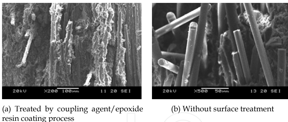
Fig. 8. SEM photos of transverse tensile fracture sections of carbon/glass hybrid fiber reinforced NASC
