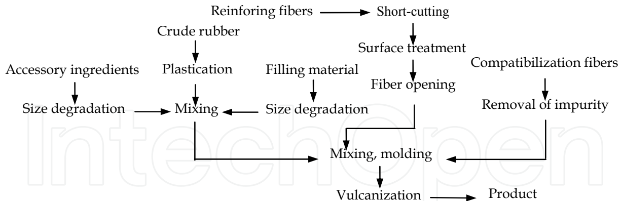
Fig. 1. A molding process of NASC
