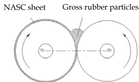
Fig. 4. The operating principle of a roller-type calender
