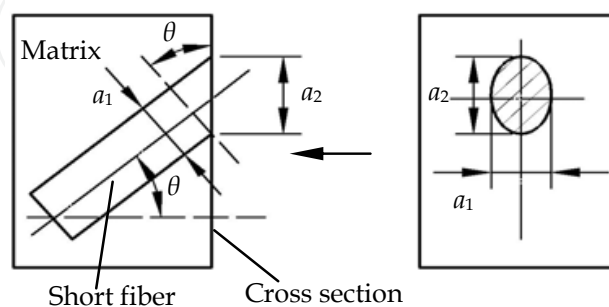
Fig. 11. A schematic diagram of the section-analysis method
