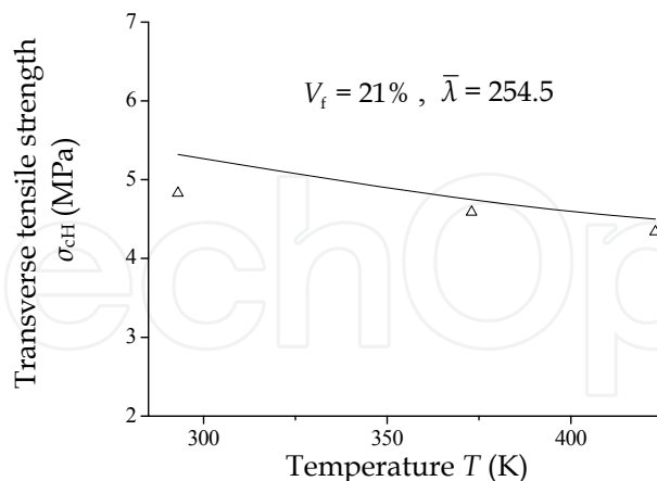
Fig. 22. Effect of temperature on transverse tensile strength
