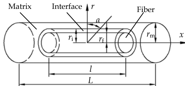
Fig. 12. A micromechanical model of NASC
