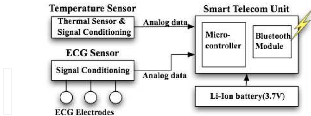
Fig. 7. Block diagram of the portable vital sensing unit (ECG and body temperature meter)
