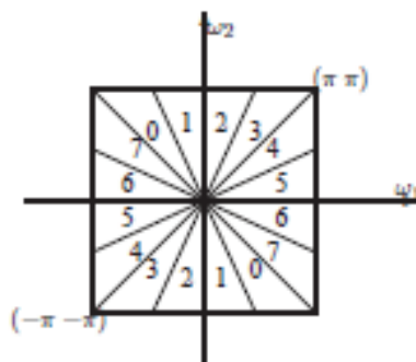
Fig. 9. DFB frequency partitioning with l=3
