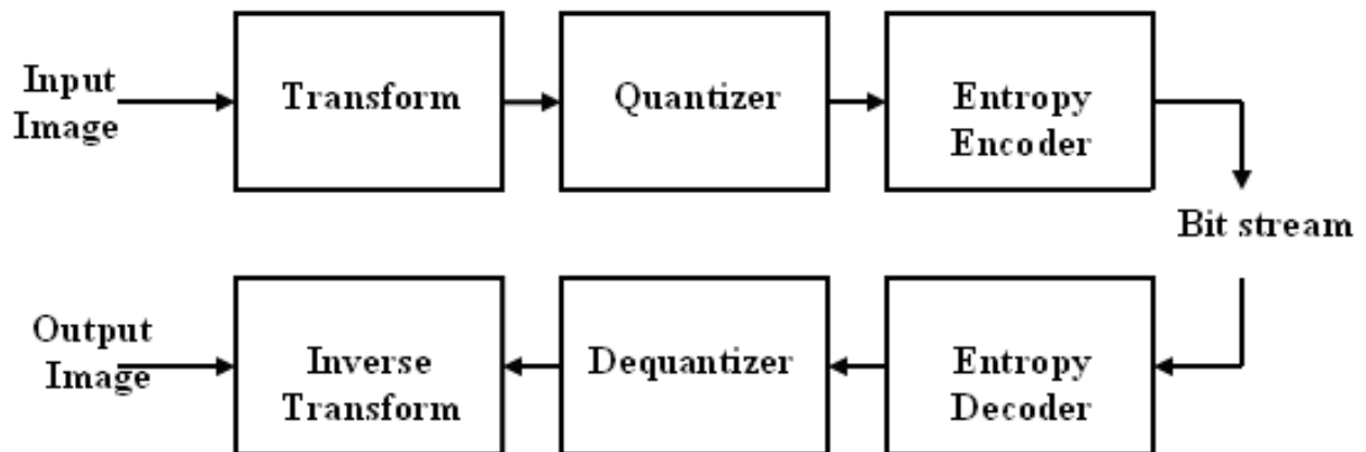
Fig. 6. Transform based image compression
