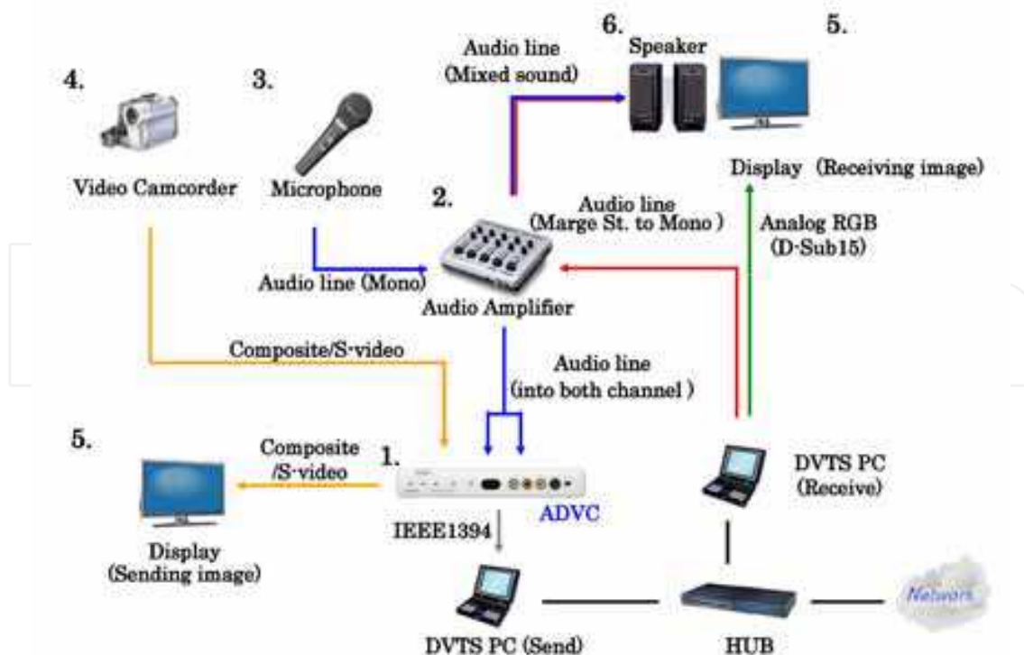
Fig. 3. Standard configuration: 1. Analog-Digital Video Converter (ADVC), 2. Audio amplifier, 3. Microphone, 4. Video camera, 5. Display, 6. Loud speaker
