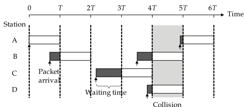
Fig. 4. Packet transmissions in a Slotted ALOHA system
