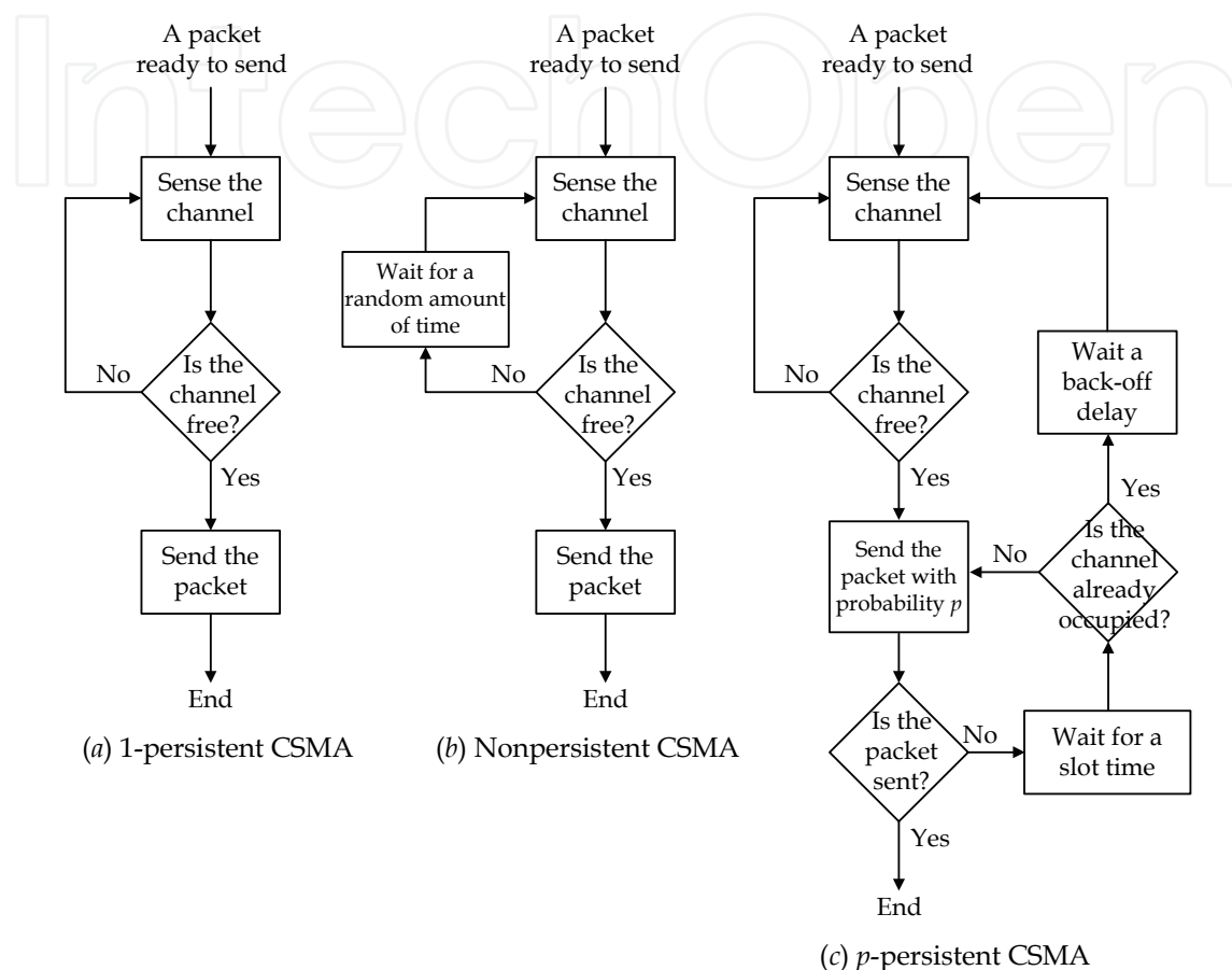
Fig. 7. Flow diagrams for CSMA systems
