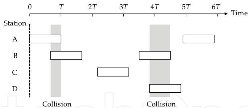
Fig. 1. Packet transmissions in a Pure ALOHA system
