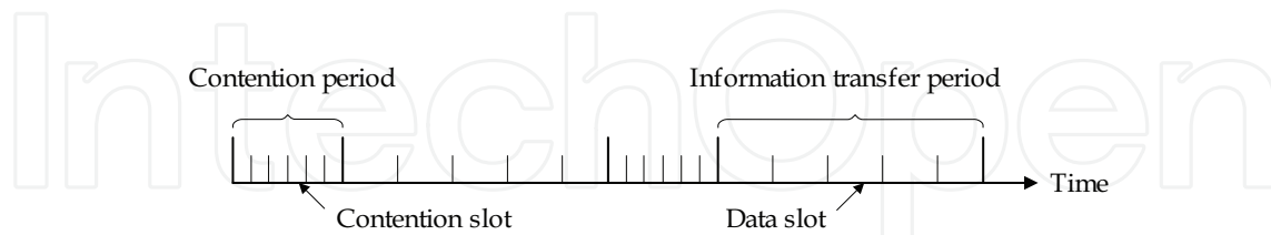
Fig. 13. A frame structure of MAC protocols
