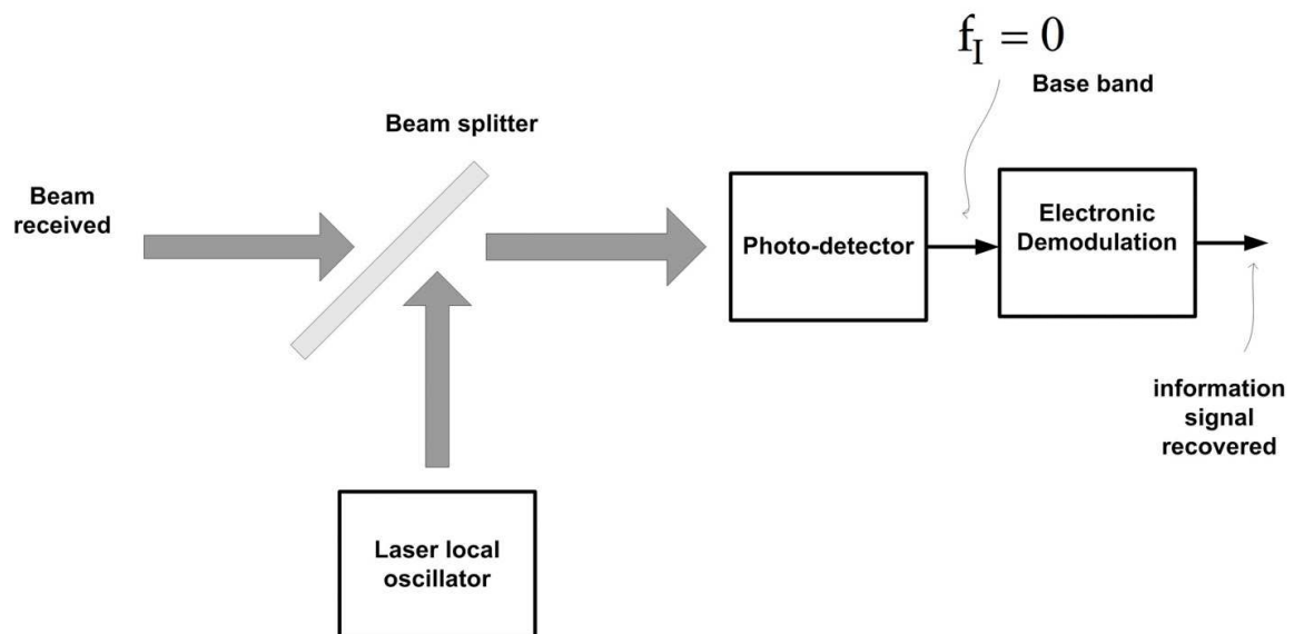
Fig. 5. Optical homodyne receiver
