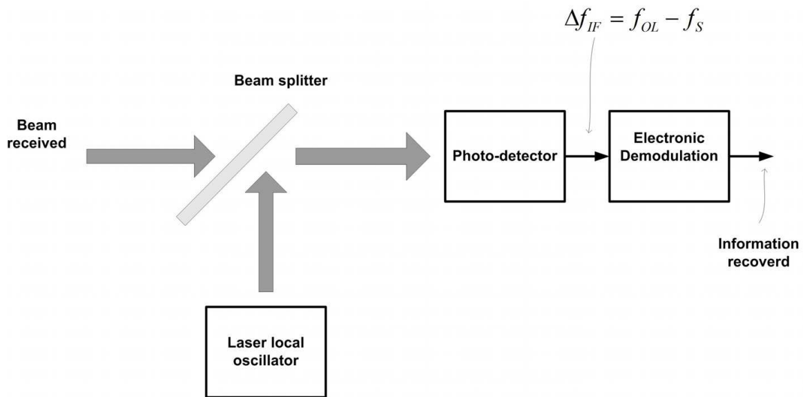
Fig. 4. Optical heterodyne receiver
