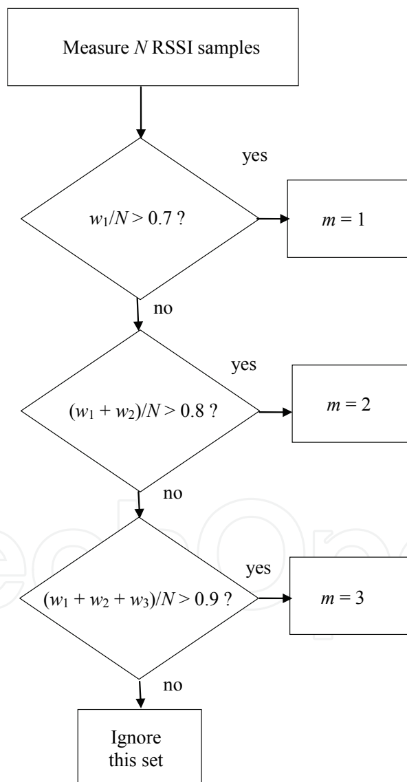
Fig. 2. Weighted-mean filter (3) algorithm
