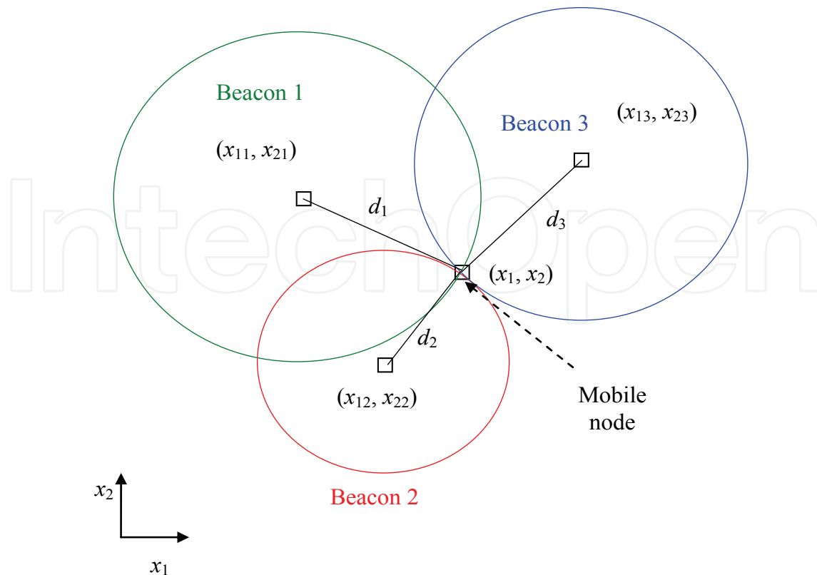
Fig. 1. Trilateration approach example for three beacons
