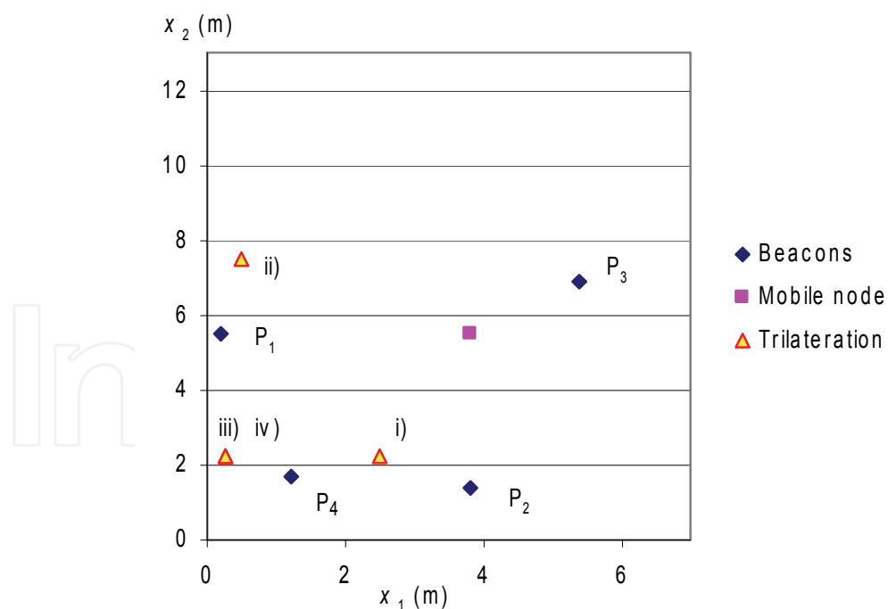
Fig. 7. Trilateration example using ZigBee commercial hardware
