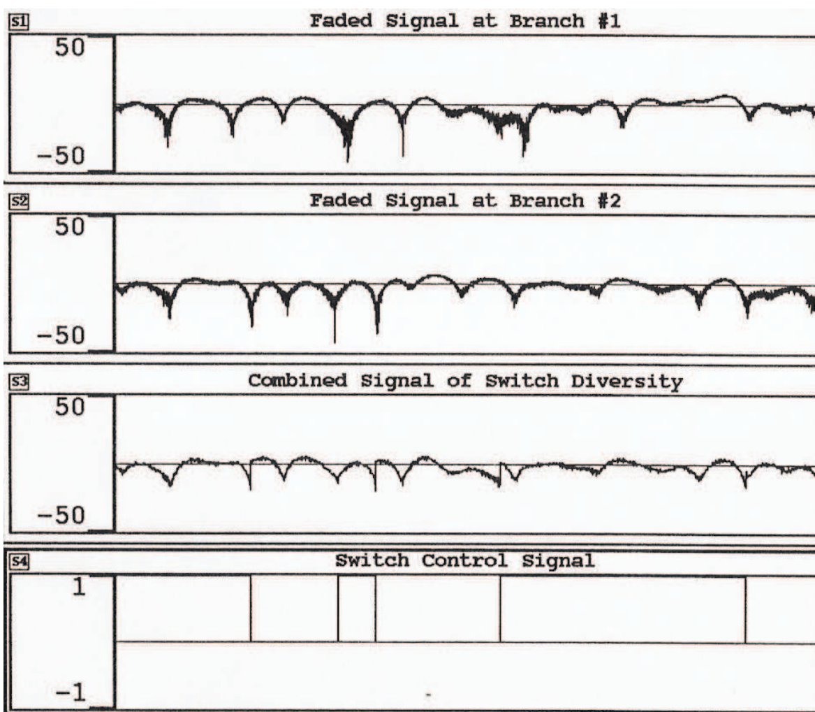
Fig. 3. Fading Signal Envelopes in Diversity Branches ( L=2 )
