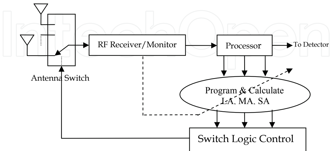
Fig. 5. Antenna Switch Diversity for Wireless Channel
