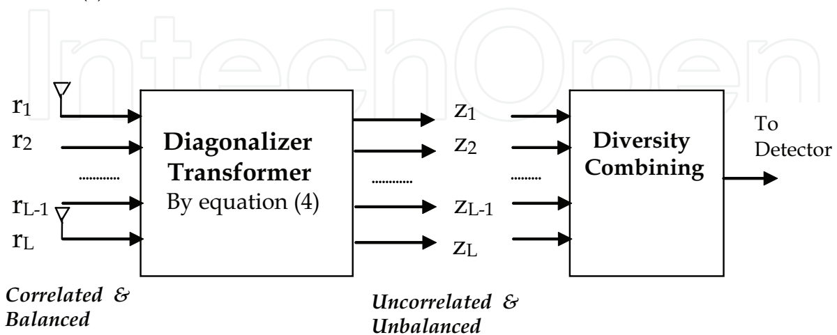
Fig. 1. Diagonalizer (Transformer) Block Diagram
