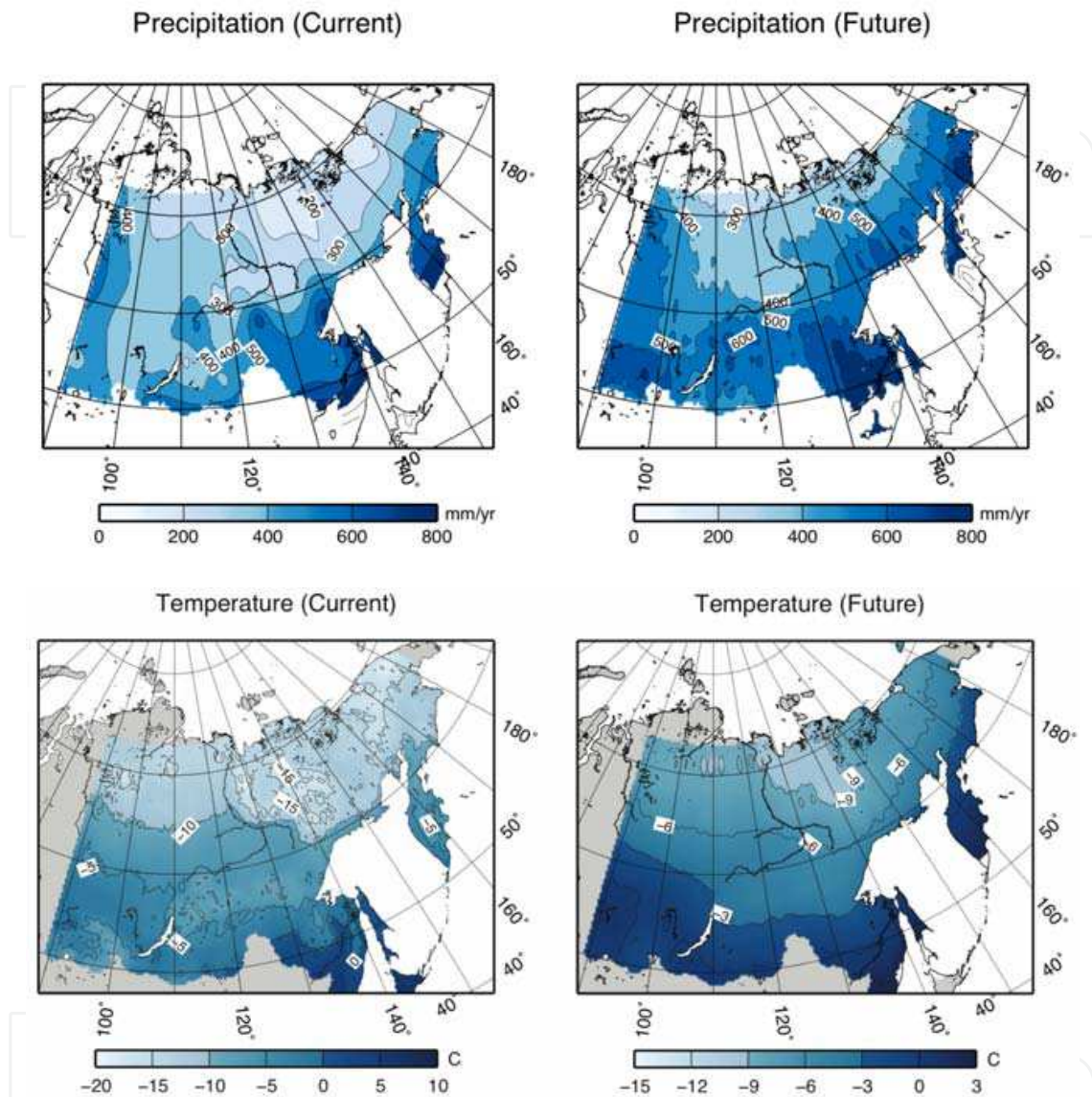
Fig. 1. Comparison of spatial distribution of mean annual precipitation (top) and mean annual air temperature (bottom) between Current (1986-2004, left-hand side panel) and Future (2081-2100, right-hand side panel).
