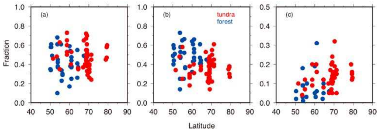
Fig. 3. Distribution of LE/R_n (a), H/R_n (b), and G/R_n (c) of different vegetation types across a latitudinal range. They are arranged based on the data of Eugster et al. (2004), Baldocchi et al. (2000), Beringer et al. (2005), and Bernhofer et al. (2003)
