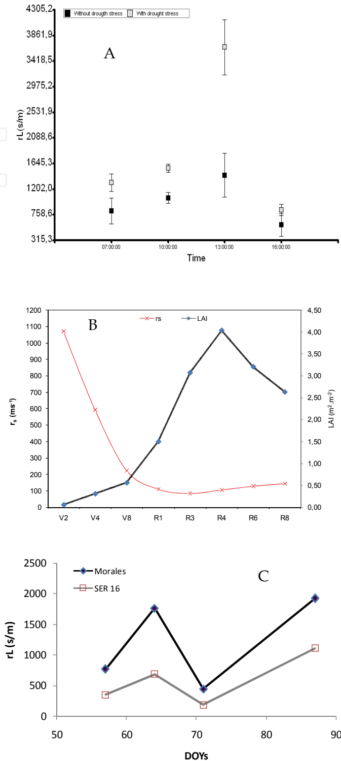
Fig. 3. Relationship between A. Changes in the stomatal resistance during the day with and without drought stress in Phaseolus vulgaris L. genotype 'Morales'. B. Surfaces resistance and Leaf area index, and C. Stomatal behaviour represented in stomatal resistance ( r_L ) under drought stress conditions for two common bean genotypes -'Morales' lest drought tolerant and 'SER 16' drought stress tolerant.
