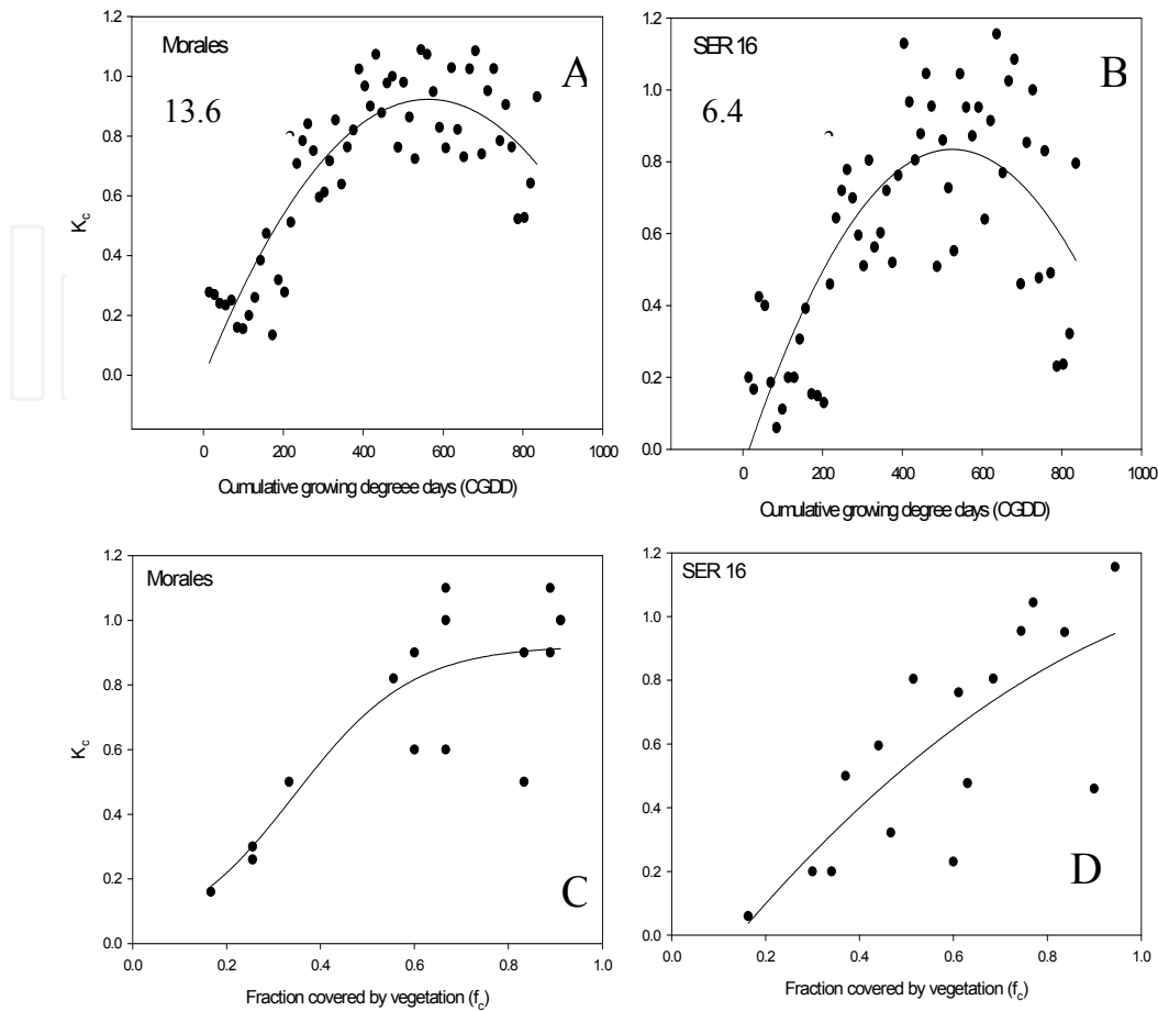
Fig. 1. Crop coefficients ( K_c ) as related to cumulative growing degree days (CGDD) and fraction covered by vegetation ( f_c ) for two common bean genotypes: A. Morales CGDD vs K_c , B. SER 16 CGDD vs K_c , C. Morales f_c vs K_c , D. SER 16 f_c vs K_c . The curves were fitted from growth periods V1 to R9 (Data from: Ramirez, 2007). (These data's were obtained under the project sponsored by NOAA-CREST (NA17AE1625), NASA-EPSCoR (NCC5-595), USDA-TSTAR-100, USDA Hatch Project H-402, and University of Puerto Rico Experiment Station)
