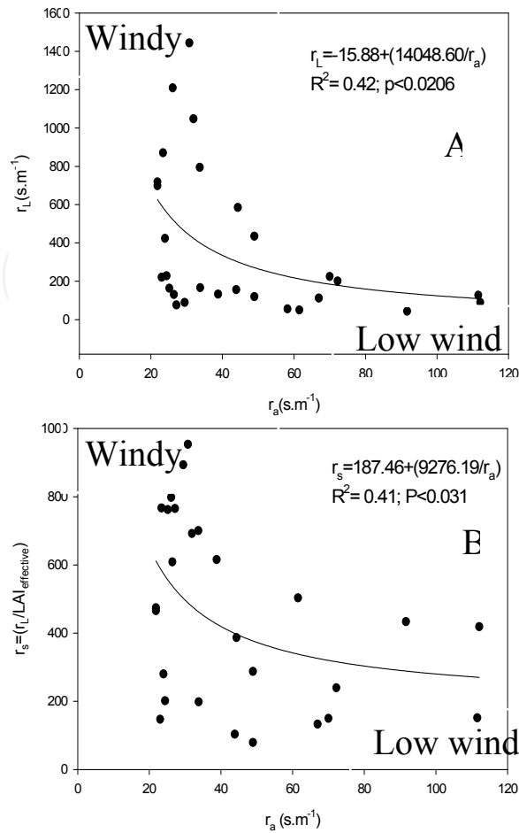
Fig. 4. Aerodynamic resistance ( r_a ) as a function of: A. Stomatal resistance ( r_L ) and B. Measured surface resistance: r_s = r_L/LAI_{effective} , (Dats from: Ramirez, 2007).
