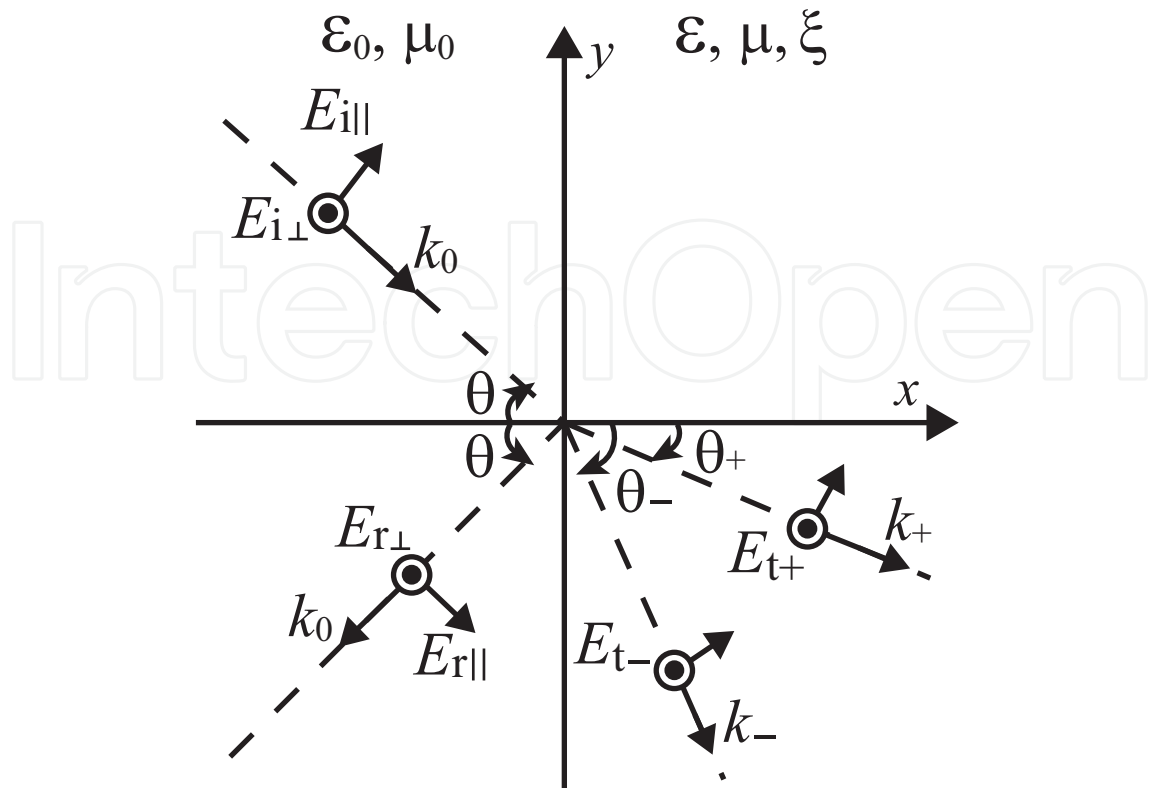
Fig. 1. Geometry of coordinate system. Incident, reflected, and transmitted waves are denoted by subscripts i, r, and t. Region x < 0 represents vacuum, and region x \geq 0 represents the chiral medium.
