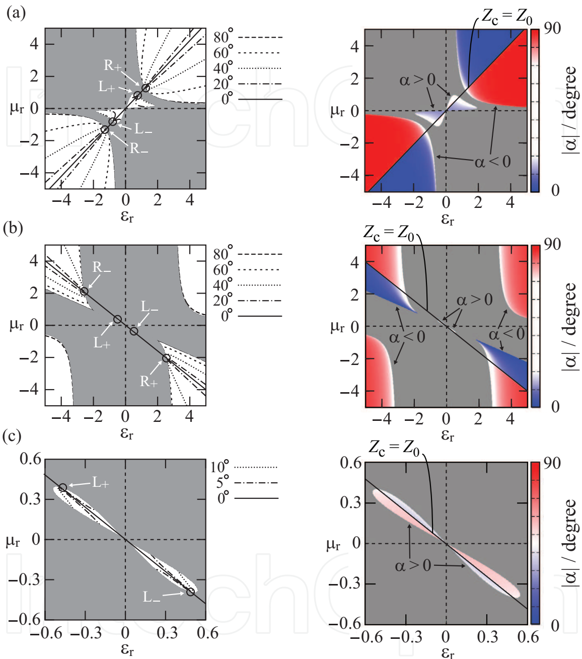
Fig. 3. No-reflection conditions (a) for \zeta_r = \zeta Z_0 = 0.2 and (b), (c) for \zeta_r = 1.5 . [Note that the scale of (c) is different from other figures.] (left panels); contour lines of no-reflection angles. L_+ and R_+ ( L_- and R_- ) represent the no-reflection conditions for LCP and RCP waves written in Eq. (48) [Eq. (49)], respectively. (right panels); ellipticity \alpha of incident polarization for which no-reflection condition is satisfied. Sign of \alpha is reversed if sign of \zeta_r is reversed. No-reflection conditions do not exist in gray region.
