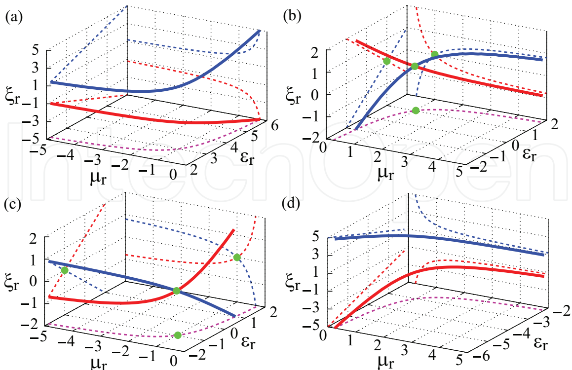
Fig. 4. Relations among \varepsilon_r , \mu_r , and \zeta_r that satisfy no-reflection condition for CP waves: (a), (b) relations given by Eq. (48), and (c), (d) relations given by Eq. (49). Red (blue) solid lines represent no-reflection condition for LCP (RCP) waves. Dashed lines are projections of solid lines on each plane. Green solid circles correspond to (b) vacuum and (c) anti-vacuum.
