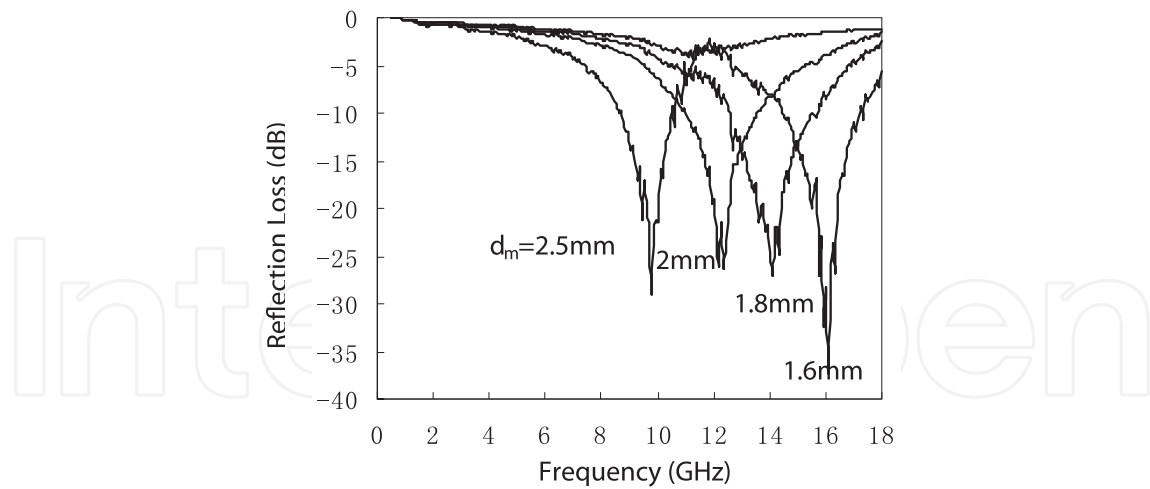
Fig. 15. Frequency dependence of reflection loss for \text{Nd}_6\text{Fe}_{91}\text{B}_3 compositions with different matching thickness
