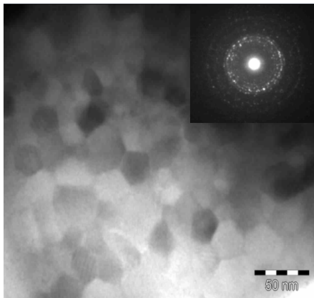
Fig. 8. TEM micrograph and diffraction patterns of the heat treated \text{Nd}_x\text{Fe}_{94-x}\text{B}_6 ( x=9.5 ) melt-spun ribbons
