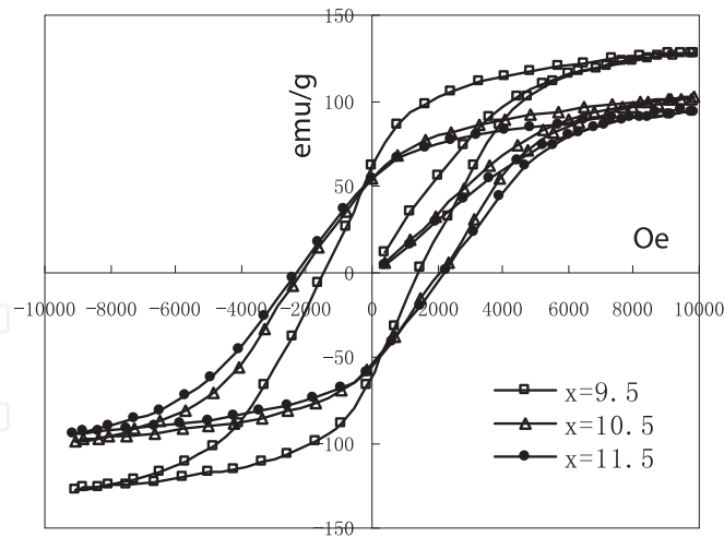
Fig. 7. Magnetic hysteresis loops for \text{Nd}_2\text{Fe}_{14}\text{B}/\alpha\text{-Fe} nanocomposites powder with different Nd content
