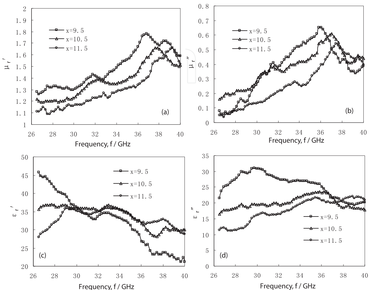
Fig. 9. The frequency dependencies of the complex relative permeability and permittivity of resin composites \text{Nd}_x\text{Fe}_{94-x}\text{B}_6 ( x=9.5, 10.5, 11.5 ):
