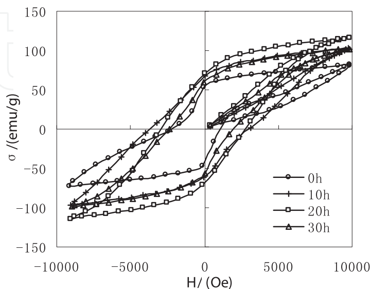
Fig. 17. Magnetic hysteresis loops for \text{Nd}_{10}\text{Fe}_{84}\text{B}_6 composite with various milling time
