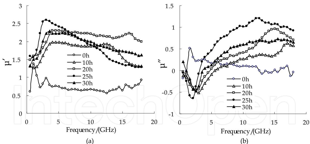
Fig. 18. The real part \mu_r' (a) and imaginary part \mu_r'' (b) of complex relative permeability against frequency for \text{Nd}_{10}\text{Fe}_{84}\text{B}_6 composite after various milling time in the 0.5-18GHz
