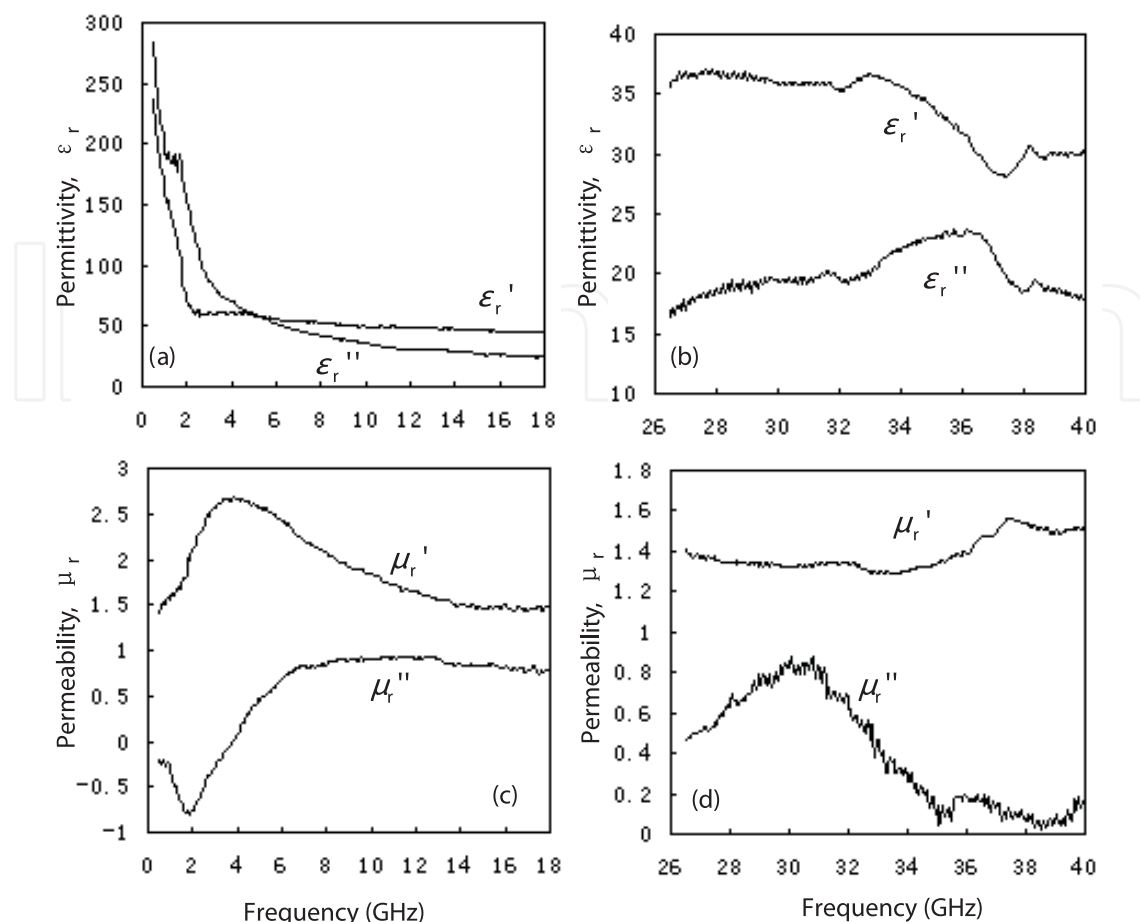
Fig. 4. The relative permittivity and permeability plotted against frequency for Nd 2 Fe 14 B/α-Fe composites in the 0.5-18 and 26.5-40GHz
