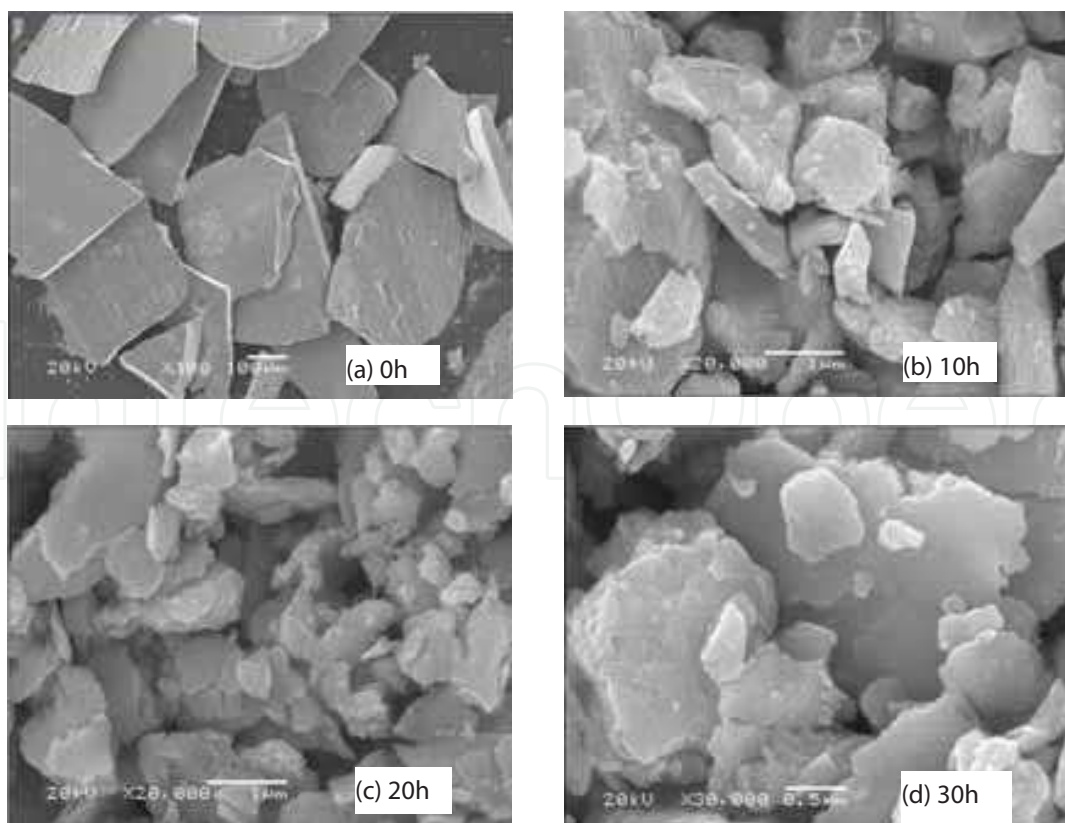
Fig. 16. SEM micrographs of \text{Nd}_{10}\text{Fe}_{84}\text{B}_6 composite with various milling time
