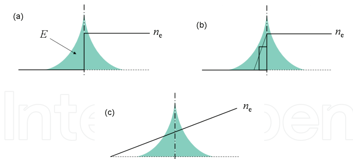
Fig. 10. Schematic view of surface waves on various models. (a) Model for ideal metal surface. (b) Bulk selvage model for metal surface. (c) Model for a discharge plasma.
