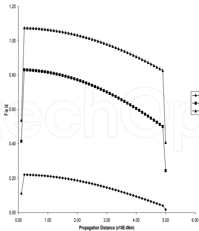
Fig. 2. The field behaviour as it propagates through the film thickness Z\mu\text{m} for mesh size = 50 when \lambda = 0.25\mu\text{m} , 0.7\mu\text{m} and 0.9\mu\text{m} .
