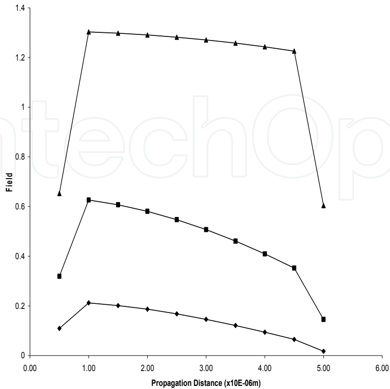
Fig. 1. The field behaviour as it propagates through the film thickness Z\mu\text{m} for mesh size = 10 when \lambda = 0.4\mu\text{m} , 0.7\mu\text{m} and 0.9\mu\text{m} .
