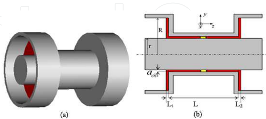
Fig. 8. (a) Model of the “dumbbell -shaped” coaxial metallic waveguide. (b) Cross-section of the model. Red region: ENZ metamaterials; Yellow region: testing sample; Grey region: metallic conductor ( R = 20\text{mm} ; r = 8.7\text{mm} ; L = 1.5R = 30\text{mm} ; L_1 = L_2 = a_{ch} = R / 20 = 1\text{mm} ). [15] (Wu et al, 2008)
