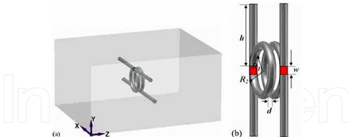
Fig. 14. (a) Perspective of the model of waveguide filled by one pair of \Omega -shaped particles. (b) The \Omega -shaped particles. Red region denotes the detecting zone, i.e., gap of the \Omega -shaped particle (Huang et al, 2009)
