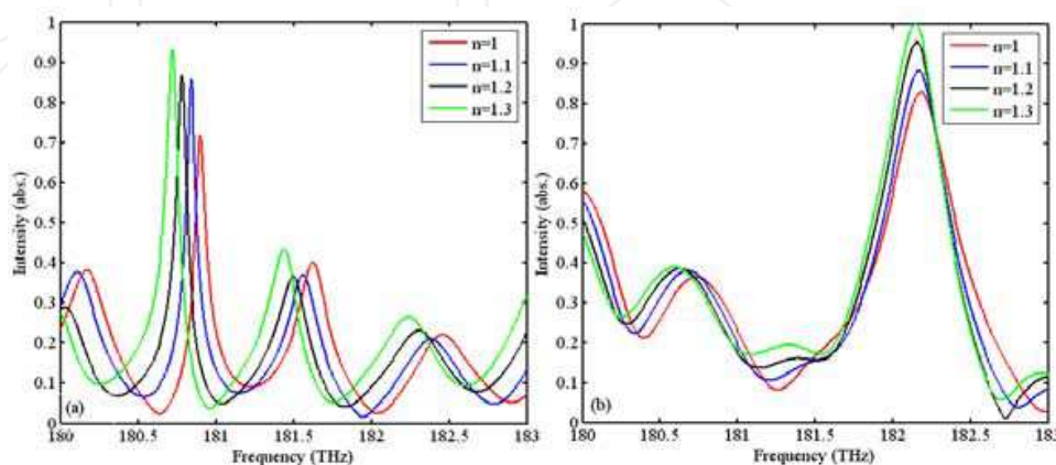
Fig. 28. Spectra for the surrounding medium with different refractive index. (a) Results for the microring cavity without metamaterial layer. (b) Results for the microring cavity with metamaterial layer
