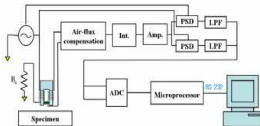
Fig. 10. Schematic diagram of the sensor system
