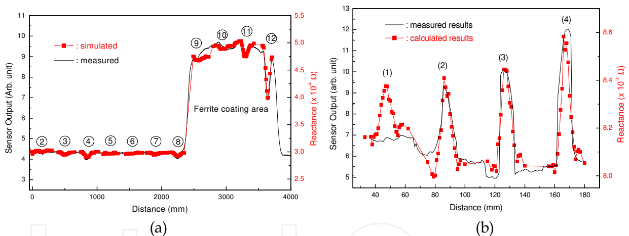
Fig. 23. Reactance simulated by FEM and output measured by manufactured sensor for (a) with and without outside ferrite sludge, (b) with nickel sleeving. The numbers from 2 to 8 are LMPs, from 9 to 12 LMPs with outside ferrite sludge at (a), and the numbers 1, 2, 3, and 4 are LMPs with nickel sleeving at (b)
