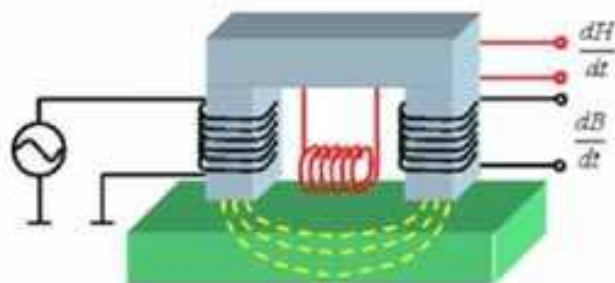
Fig. 8. Structure of the permeability sensor
