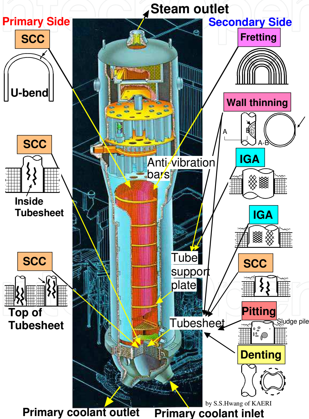
Fig. 2. The structure of SG and degradation mechanism
