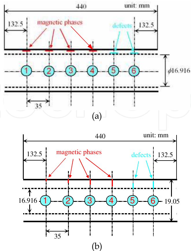
Fig. 16. Schematics of the RS for simulation of MPs and defects. (a) The numbers 1, 2, 3, and 4 are LMPs in the outer wall, while 5 and 6 are LDs in the inner one. (b) The numbers 1, 2, 3, and 4 are CMPs in the outer wall, while 5 and 6 are CDs in the inner one
