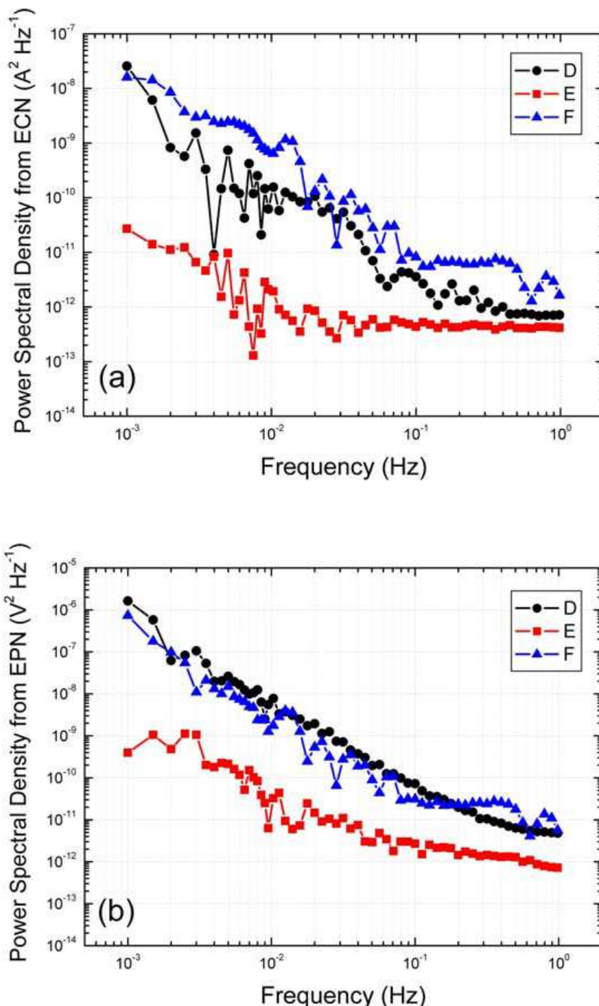
Fig. 8. Plots of the PSD vs. the frequency calculated from each time record of (a) the ECN and (b) the EPN by the FFT algorithm at points D, E and F in Fig. 5(b)
