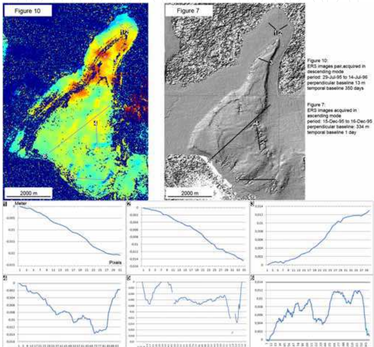
Fig. 13. Evaluation of displacements through cross sections. The ERS Interferogram is characterized by a perpendicular baseline of 13 m and a temporal baseline of 350 days. The altitude of ambiguity is 770 m and the Lisan is only covered by 1/8 of topographic fringe.
