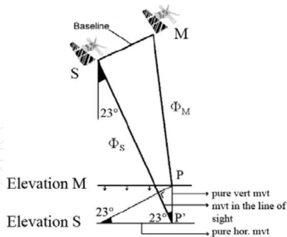
Fig. 6. Principle of DInSAR for deformation measurement. As an example, 23° is the incidence angle for ERS satellites.
