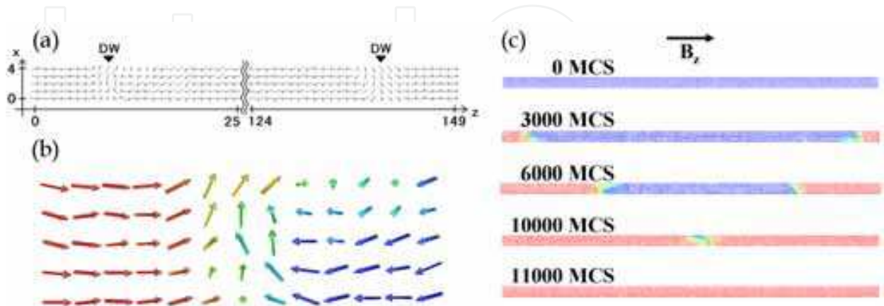
Fig. 21. (a) Snapshot of the spin structure during reversal magnetic field for the rectangular cluster at t=3000 MCS after the magnetic field was applied. (b) Enlarged view of snapshot of the spin structure around the left side DW in (a). (c) Spin snapshots on each MCS; 0 MCS, 3000 MCS, 6000 MCS and 10000 MCS.
