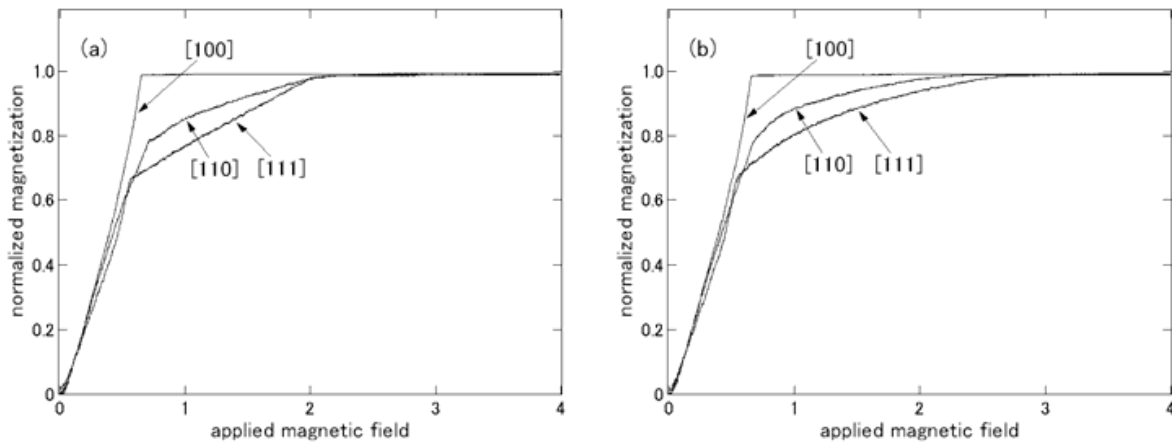
Fig. 14. Magnetization as a function of applied magnetic field along the [100], [110] and [111] directions for a spherical cluster using (a) H_1 = H_J + H_D + H_{A\_macro} + H_B and (b) H_2 = H_J + H_D + H_{A\_micro} + H_B .
