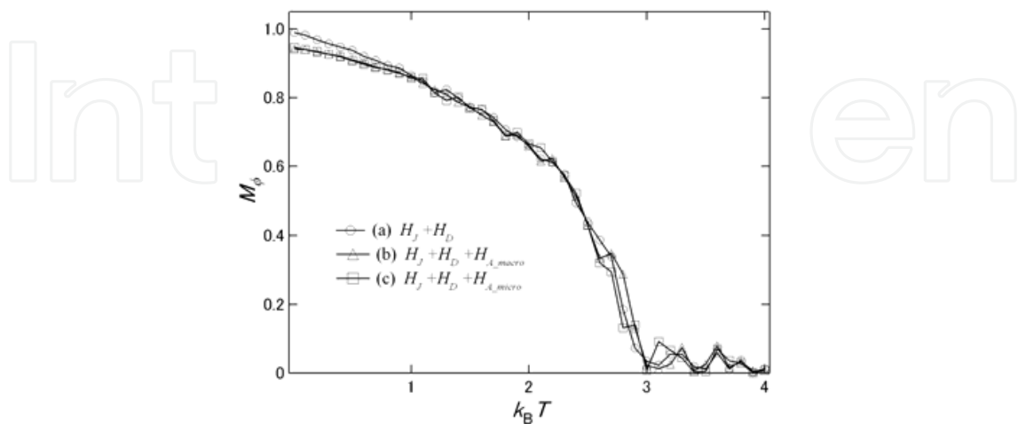
Fig. 10. Closure domain parameter M_\phi as a function of temperature k_B T for a cylindrical cluster using Hamiltonian; (a) H_J+ H_D , (b) H_J+H_D+H_{A\_macro} , (c) H_J+H_D+H_{A\_micro} .
