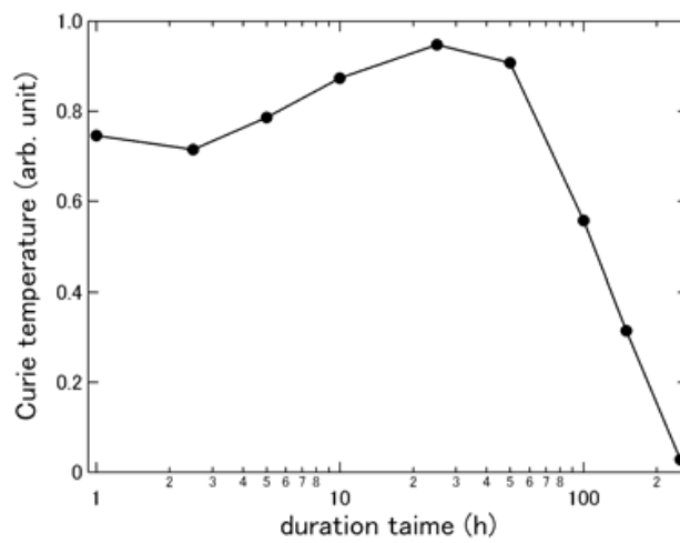
Fig. 34. Duration time dependence of Curie temperature.
