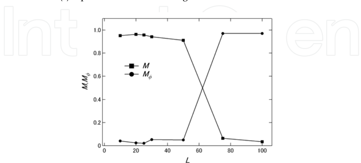
Fig. 7. Variation of M and M_\phi depending on square cluster size with L .
