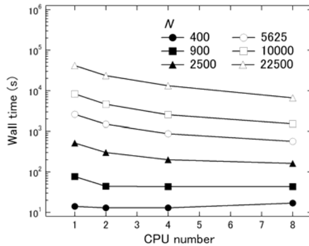
Fig. 3. Wall time during 1000 MCS depending on CPU number for each size cluster ( N=L^2 ).
