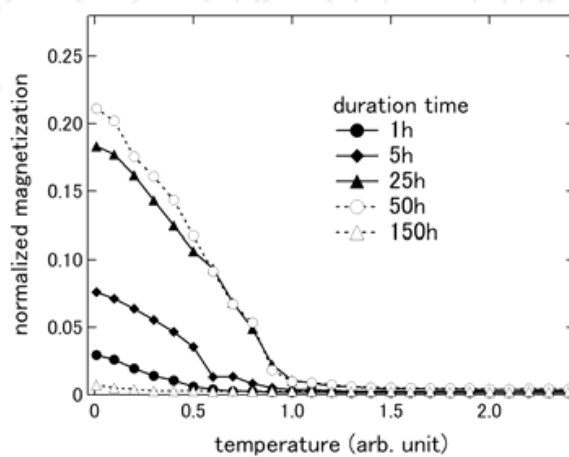
Fig. 31. Temperature dependence of calculated magnetization for each duration time
