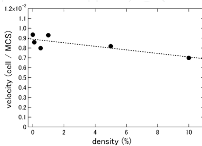
Fig. 25. DWD velocity changes with magnetic impurity densities.
