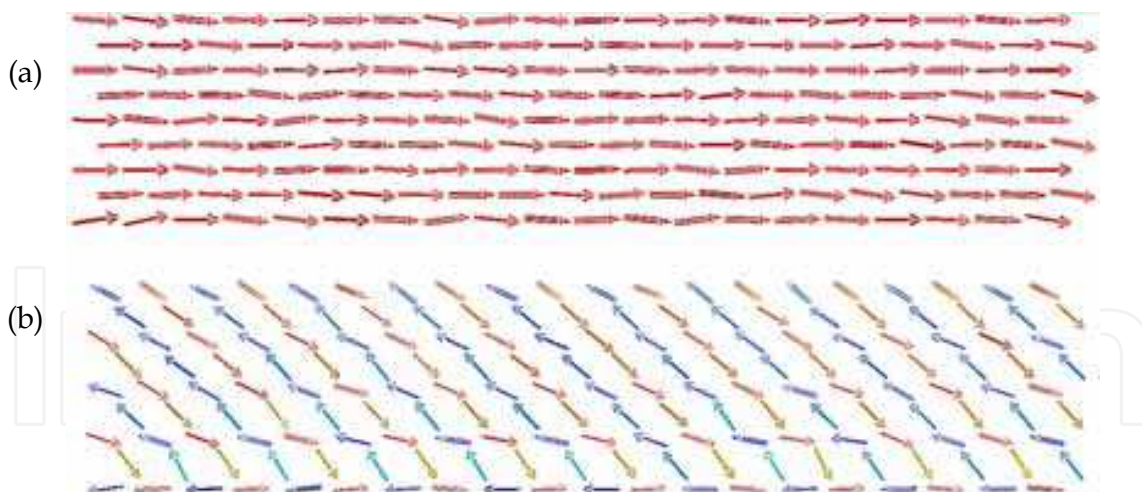
Fig. 9. Spin snapshots for a part of rectangular clusters of Eu chalcogenides with (a) J_1=0.3, J_2=-0.1 and (b) J_1=0.1, J_2=-0.3 .
