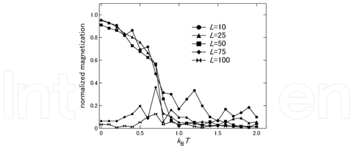
Fig. 5. Temperature dependence of normalized magnetization M for different size square clusters.
