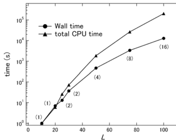
Fig. 4. Total CPU time and wall time on calculation at a fixed temperature for each size cluster. Numbers in brackets ( ) show the CPU numbers for parallel calculation.
