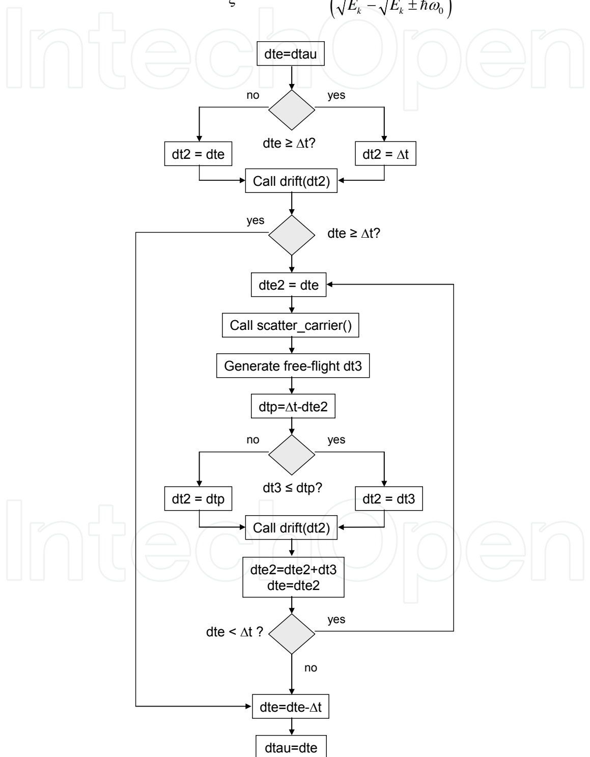
Fig. 12. Free-flight-scatter procedure within one time step.
