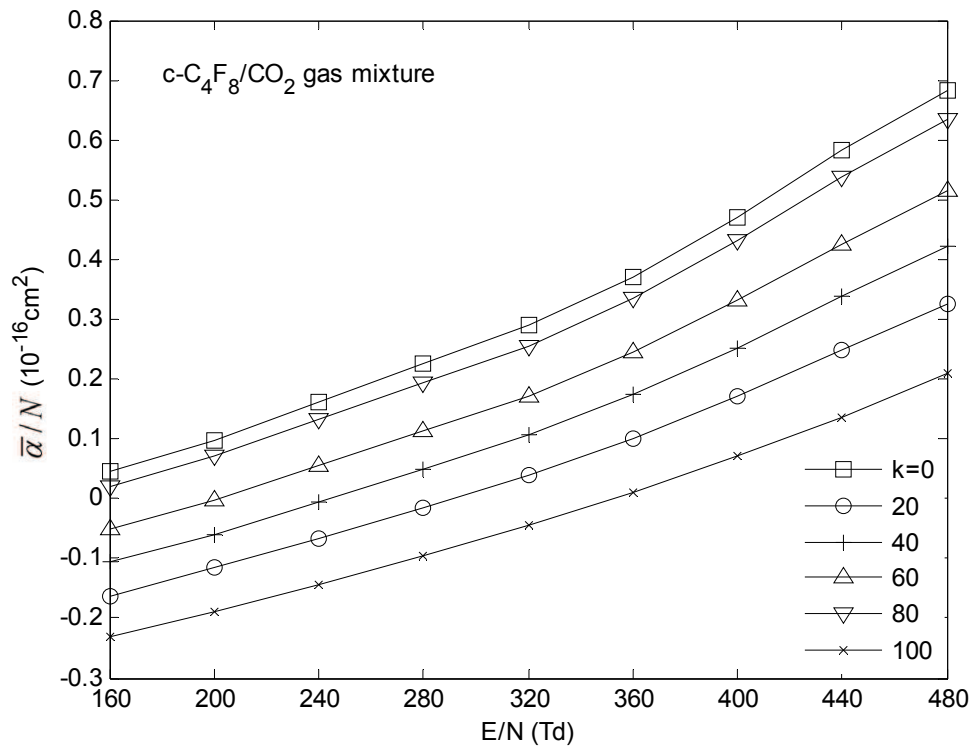
Fig. 2.13 \bar{\alpha} / N in c-C 4 F 8 and CO 2 gas mixtures as a function curve of E/N at different mixture ratio
