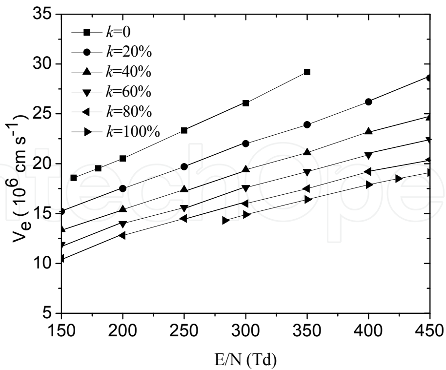
Fig. 2.14 The electron drift velocity V_e as function of E / N in c-C 4 F 8 /CO 2 mixtures at different c-C 4 F 8 gas mixture ratios k
