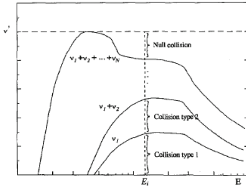
Fig. 2.2 Legend of traditional null collision Monte Carlo method
