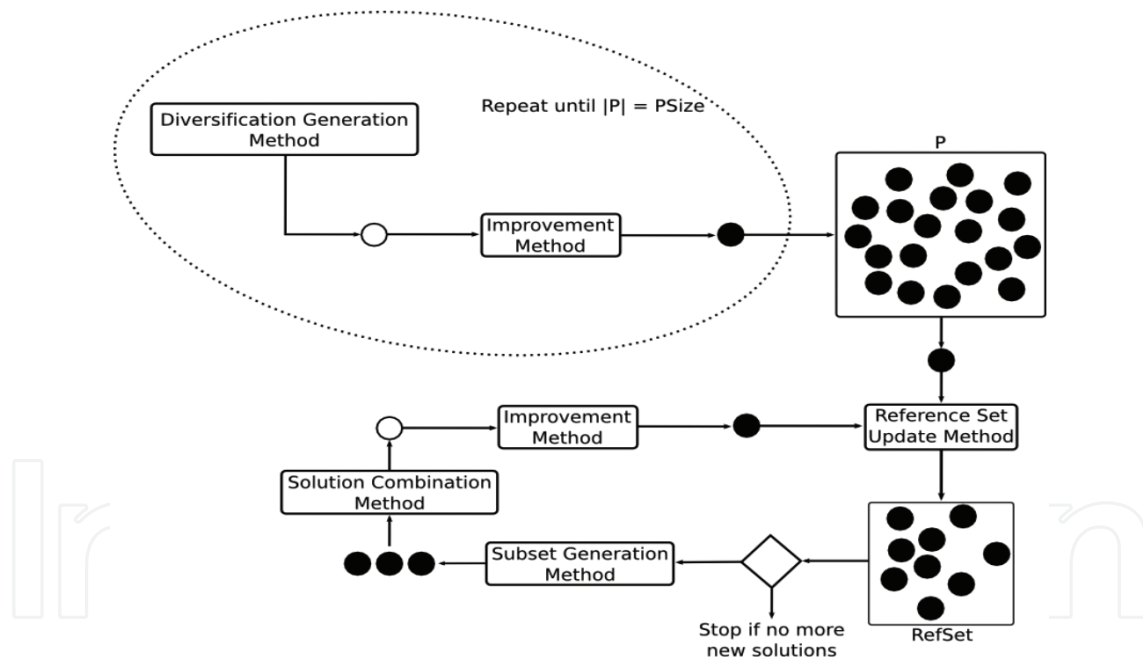
Fig. 5. Overview of Scatter Search algorithm.
