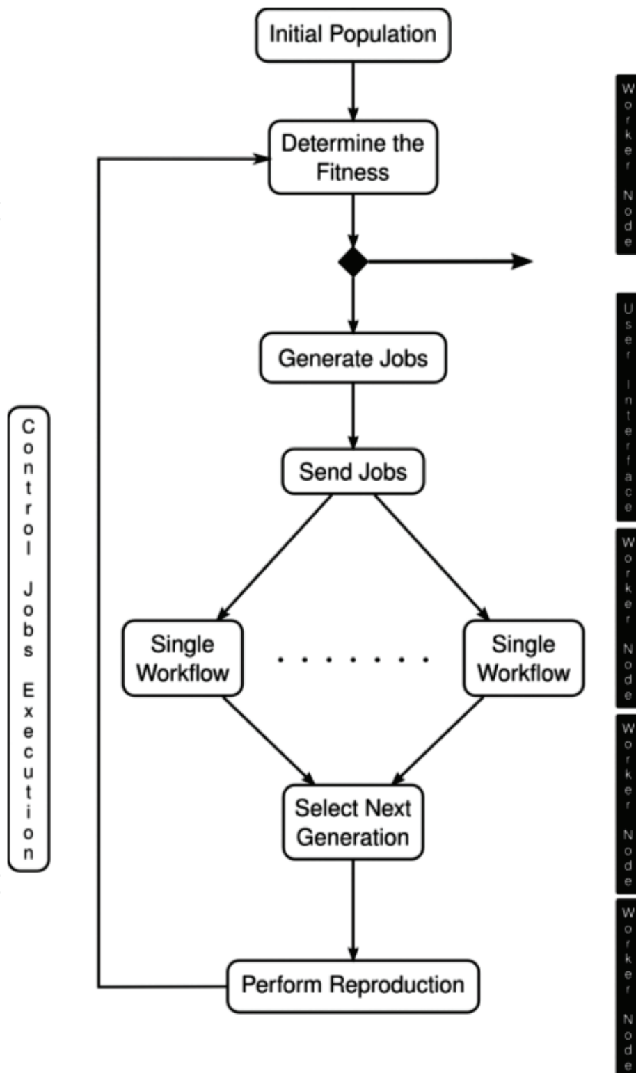
Fig. 4. Overview of a GA on the grid.
