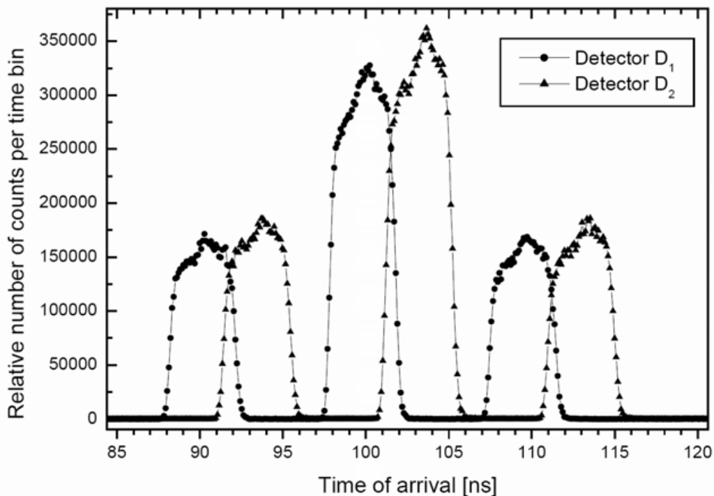
Fig. 7. Time of arrival for pulse in a 15-m time-multiplexing interferometer (circles detector D 1 , triangles D 2 ). Photons arrive in 3 time windows separated by 10 ns (corresponding to the arm length difference of 2m): the leftmost peak photons taking short-short paths, the rightmost peak photons taking long-long paths. Interference occurs only in the middle (long-short, short-long) time window.
