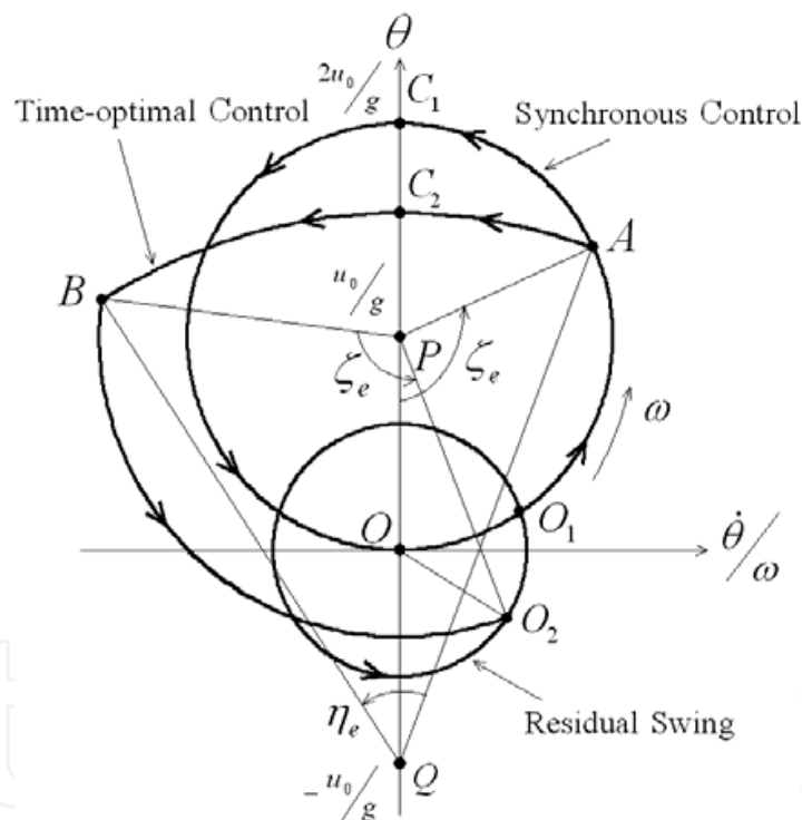
Fig. 16. Time trajectory of feed forward control using false natural period
