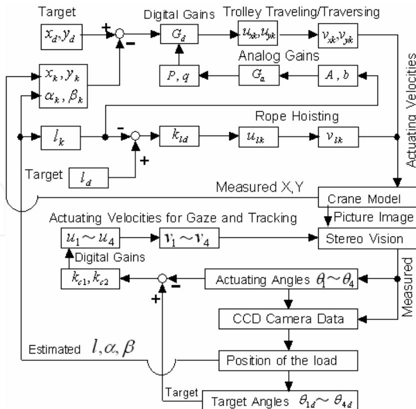
Fig. 6. Block diagram
