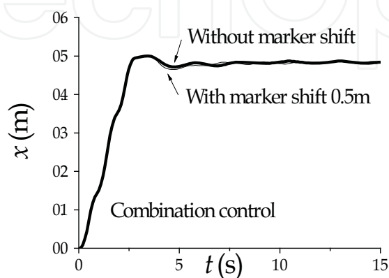
Fig. 27. Swing amplitude for arbitrary marker position
