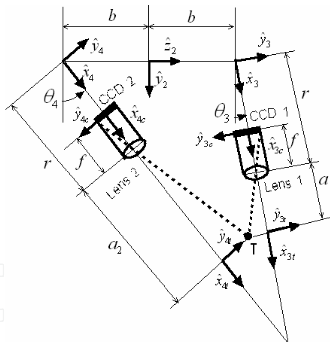
Fig. 3. Camera coordinates and optical axes
