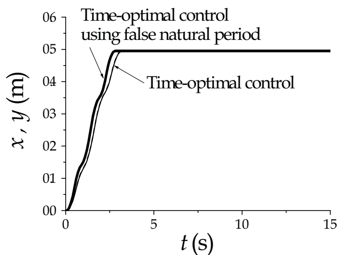
Fig. 20. Trolley transportation
