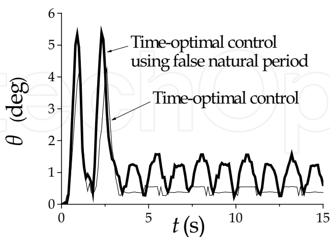
Fig. 20. Trolley transportation
