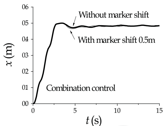
Fig. 26. Trolley transportation for arbitrary marker position
