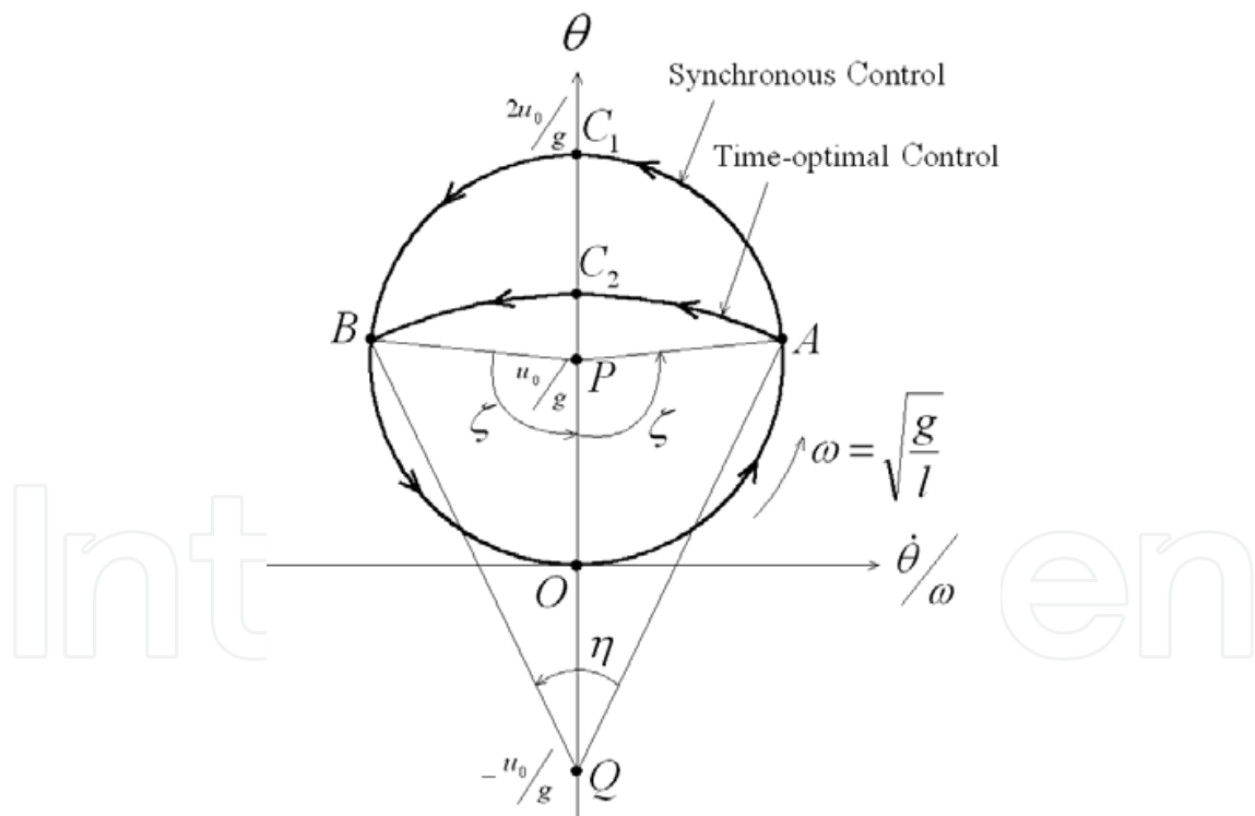
Fig. 14. Time trajectory of feed forward control
