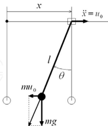
Fig. 13. Crane load under trolley's acceleration
