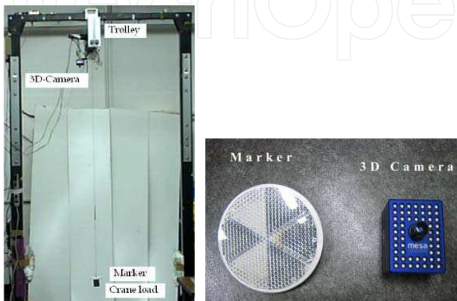
Fig. 12. Photograph of 3D-camera and marker
