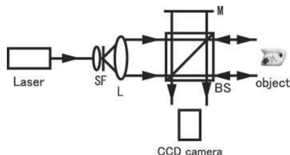
Fig. 2. Experimental setup: L, lens; SF, spatial filter; BS, beam splitter; M, mirror.
