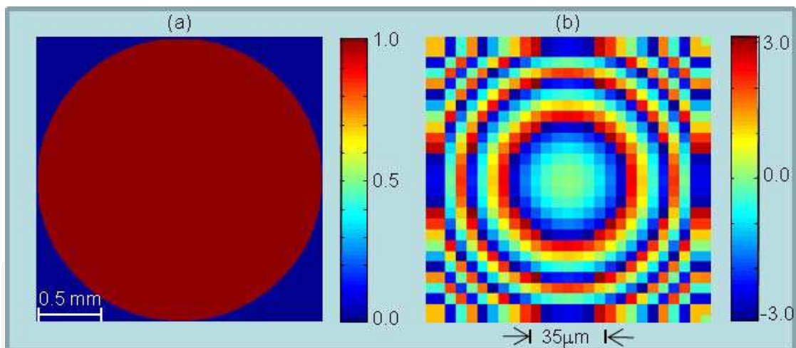
Fig. 28. (a) Amplitude of the reconstructed object field after the iteration 185, and (b) close view of the corrected version of the asymmetrical lens displayed in Fig. 26 (b).
