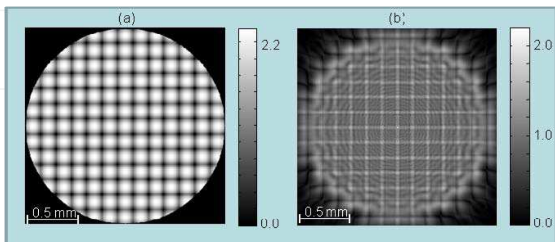
Fig. 4. (a) Phase modulation (radians) of the test object, formed by an array of micro-lenses, and (b) amplitude of the field propagated to the CCD plane.
