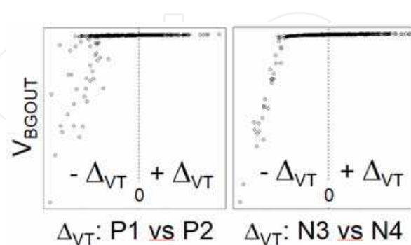
Fig. 16. Tail Traced to \Delta V_T in Bias Circuit
