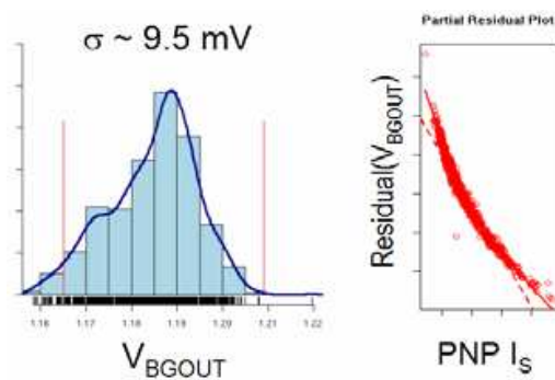
Fig. 13. Process-Only Monte Carlo Results
