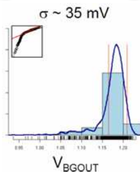
Fig. 14. Combined Process & Mismatch Monte Carlo
