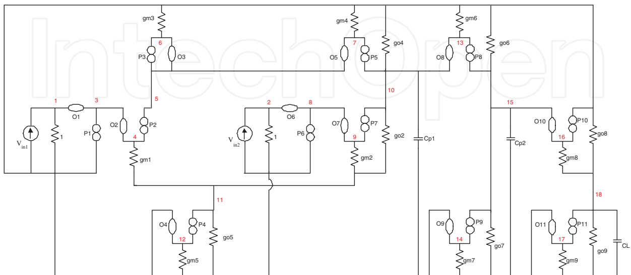
Fig. 4. Nullor equivalent from Fig. 3.
