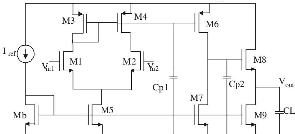
Fig. 3. Three stages uncompensated low voltage amplifier.
