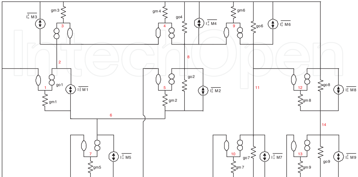
Fig. 9. Nullor equivalent from Fig. 3.
