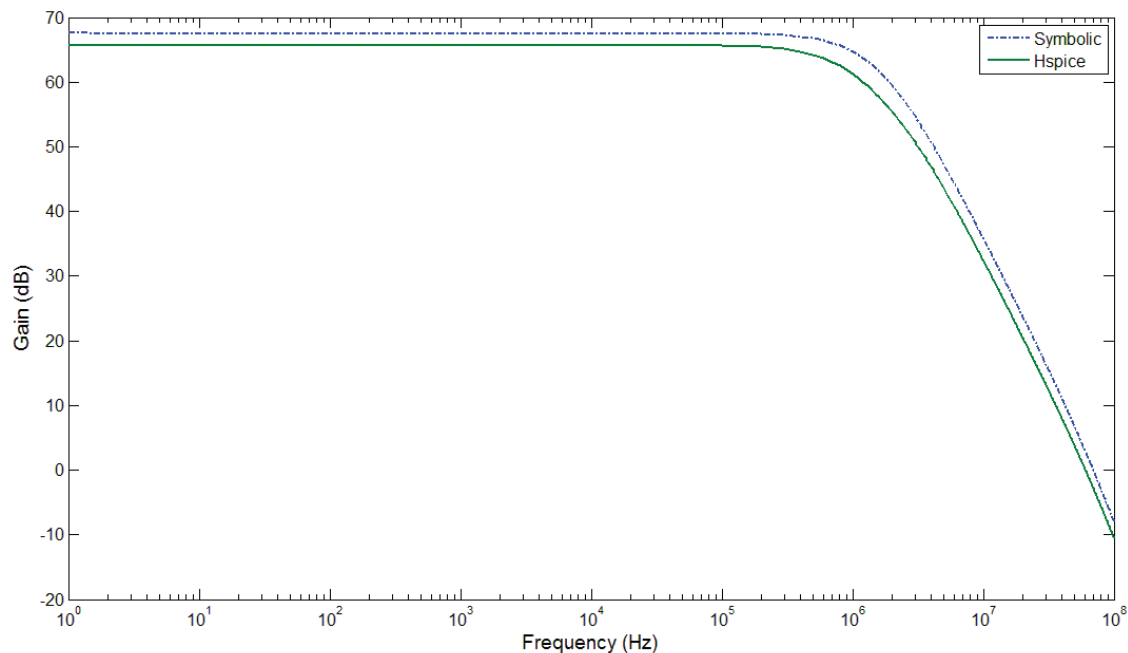
Fig. 5. Comparison between HSPICE and (4).
