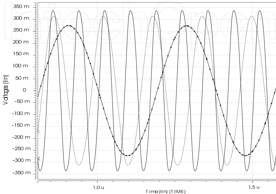
Fig. 8. Time responses of the OTRA-based sinusoidal oscillator
