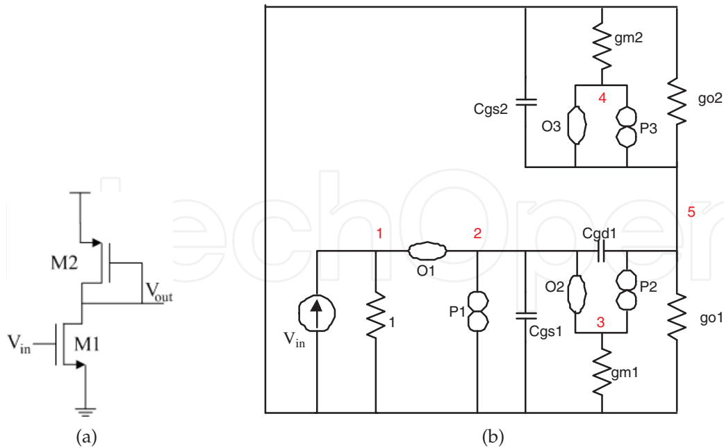
Fig. 2. (a) Low voltage amplifier with active load, and (b) Nullor equivalent.
