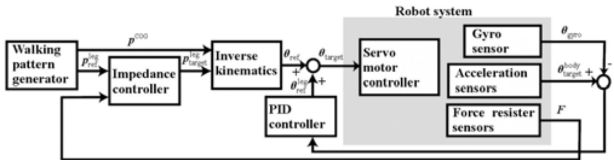
Fig. 27. Outline of walking control system for HOAP-1
