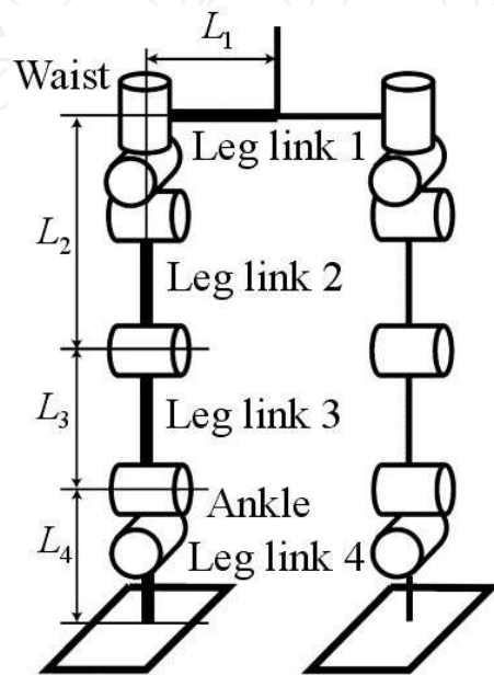
Fig. 16. Arrangement of each joint of legs
