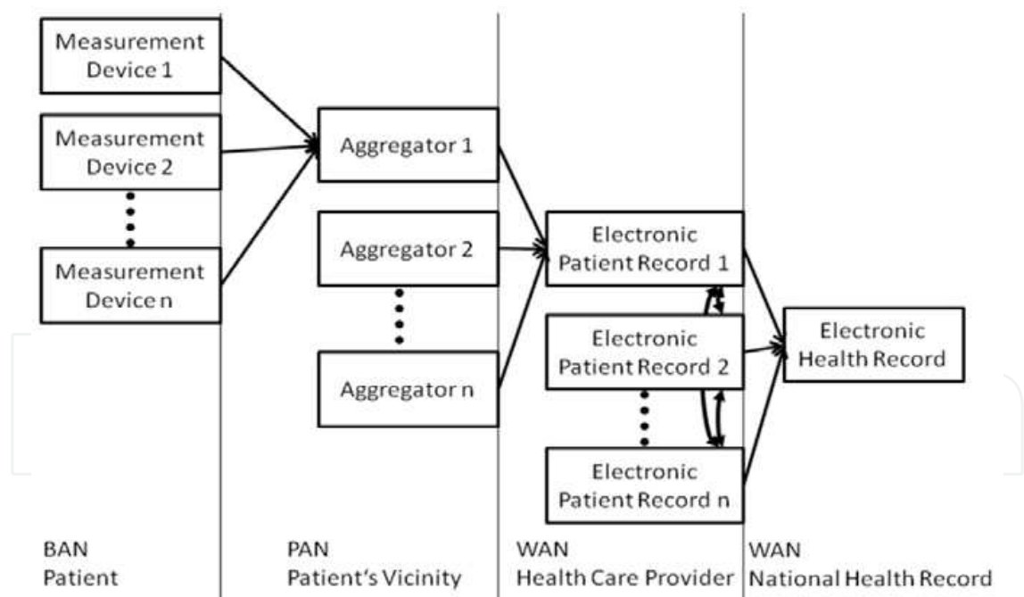
Fig. 2. Data path for cardiac rhythm disease management.
