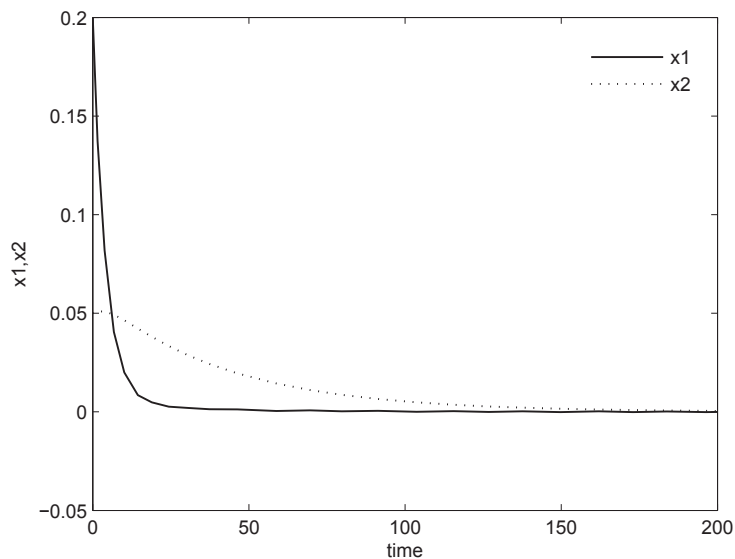
Fig. 3. The trajectories of solution of subsystem i = 2 .
