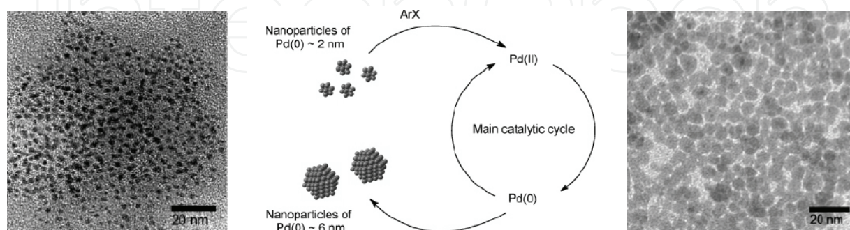
Fig. 1. TEM micrographs of the Pd-NPs in BMI.PF 6 : before catalysis ( 1.7 \pm 0.3 nm), left; after catalysis ( 6.1 \pm 0.7 nm), right. The proposed catalytic cycle for the Heck reaction promoted by Pd-NPs is indicated in the middle. Reprinted with permission from reference (Cassol et al., 2005) (Copyright American Chemical Society).
