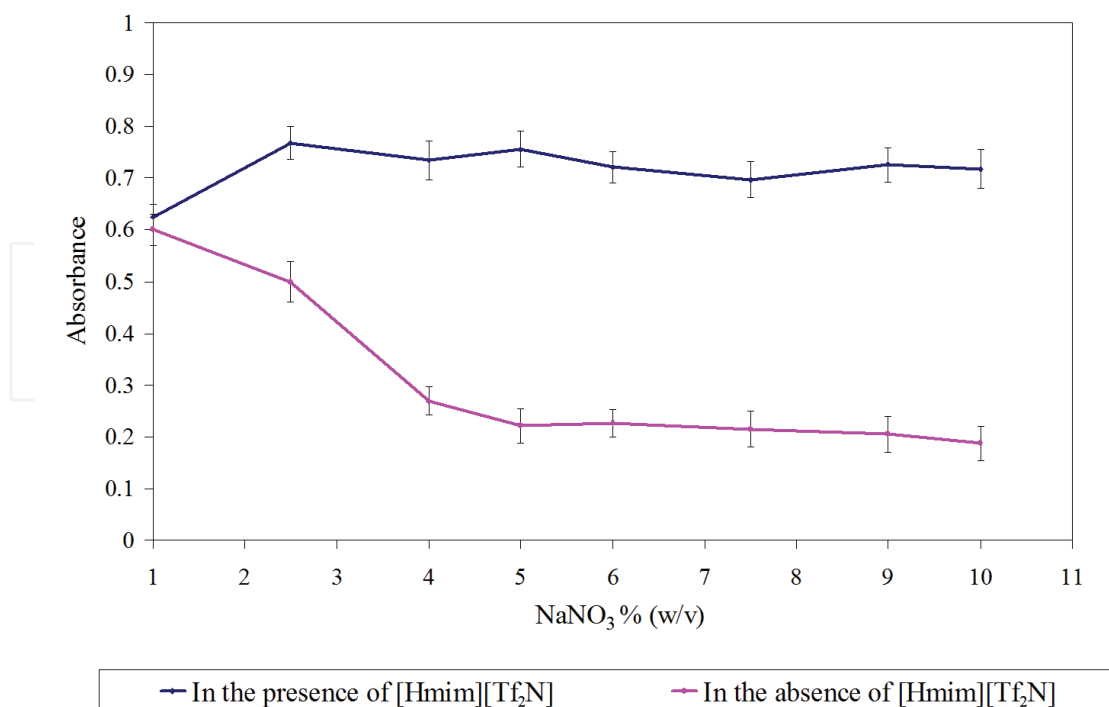
Fig. 4. Effect of NaNO 3 on the absorbance of Co-PAN complex in the range of 1-10 % (w/v). Utilized conditions: Cobalt 30 ng mL -1 , PAN 2.5×10 -5 mol L -1 , pH = 1, Triton X-114 0.05 % (w/v), [Hmim][PF 6 ] 64 mg, [Hmim][Tf 2 N] 5 mg, diluting agent 50 μL.
