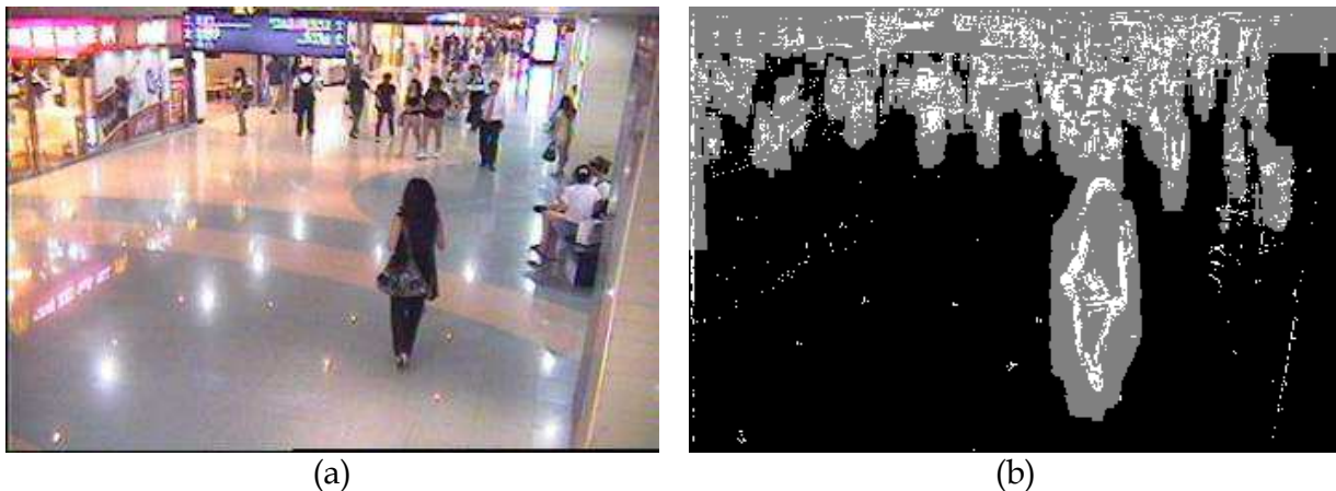
Fig. 5. Distinguishing static and non-static pixels: (a) input video frame; (b) black pixels and white pixels correspond to static and non-static pixels, respectively. Gray pixels are expanded from white pixels by morphological operations.
