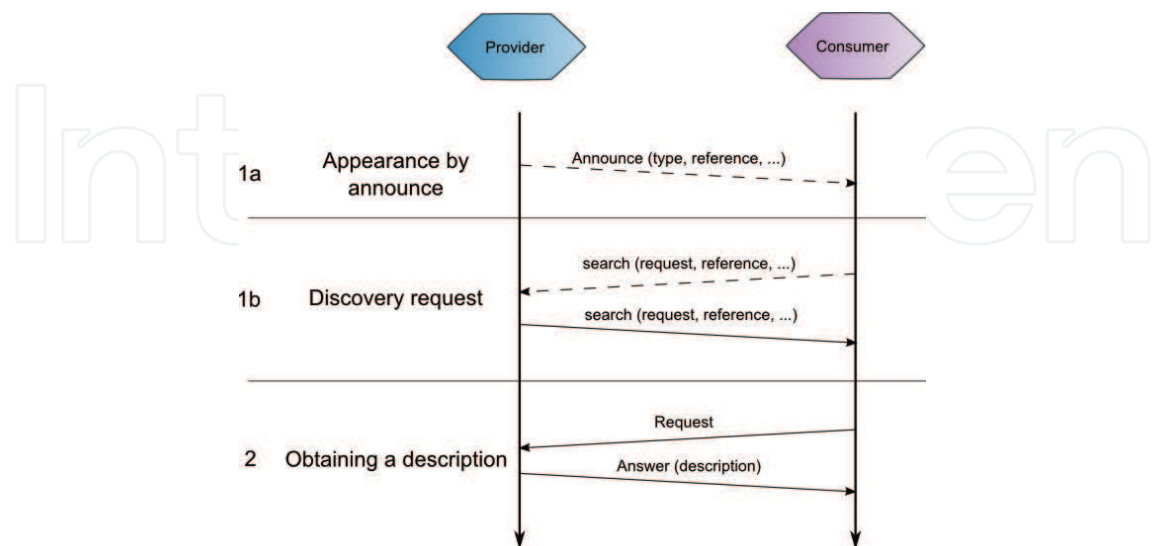
Fig. 4. Dynamic decentralized discovery : discovery and search protocols
