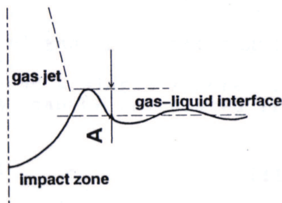
Fig. 5. A schematical representation of gas jet impact.
