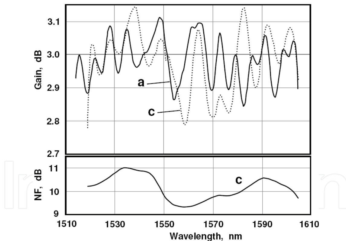
Fig. 7. Gain (top) and noise figure (bottom) spectra for a 10 km DCF Raman amplifier plus GEFs. Curve a: small launched signals and the corresponding GEF. Curves c: saturating signals with readjusted pump powers and the corresponding GEF. The pump powers are stated in Table 1 and the filter designs are illustrated in Fig. 6.
