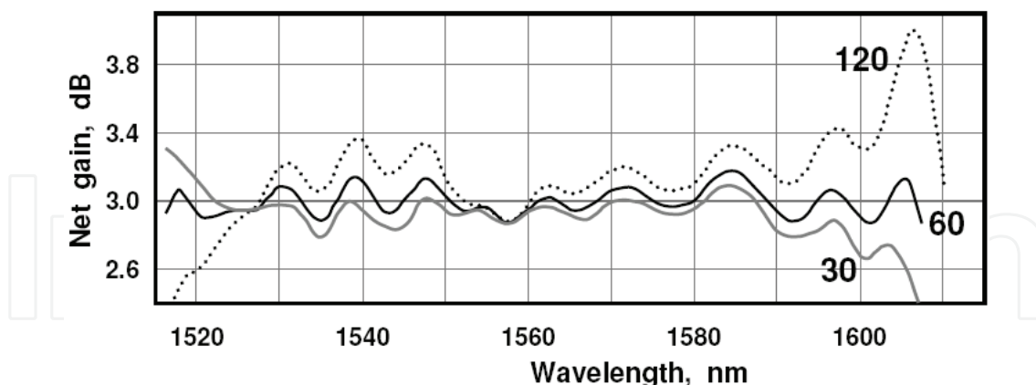
Fig. 10. Spectral variation of gain when the GEF design in Fig. 9 is placed after the DCF. The channel number and spacing are 30 channels at 400 GHz, 60 channels at 200 GHz and 120 channels at 100 GHz. The launched pump powers are as in Fig. 8.
