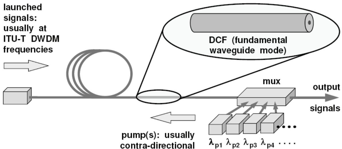
Fig. 1. Dispersion compensating fibre Raman amplifier with contra-directional multi-wavelength pumping. mux = pump-signal wavelength multiplexer.
